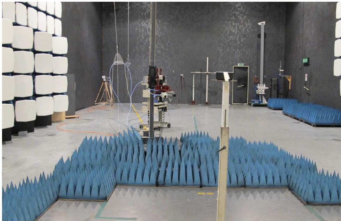
Test set up radiated emission 18 – 26.5 GHz, EUT in position X.
