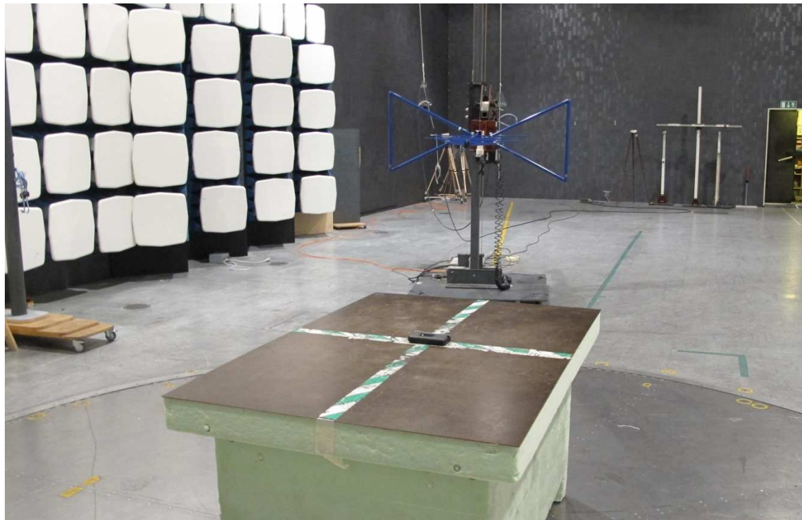
Test set up radiated emission 30 MHz – 1GHz, EUT in position Z.
