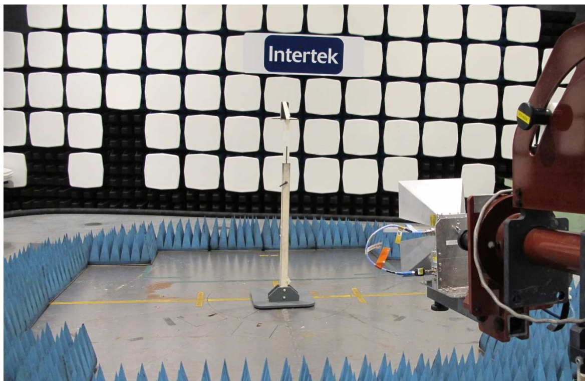
Test set up radiated emission 1 – 18 GHz, EUT in position Y.
