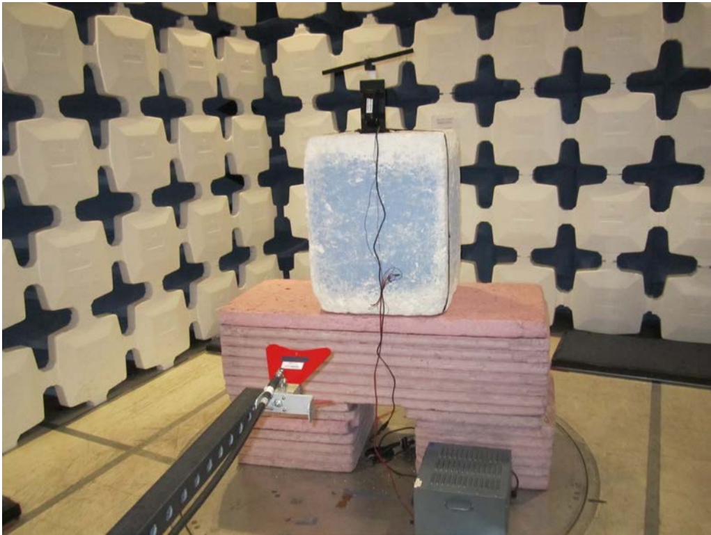
Radiated Emissions, 6-18GHz
