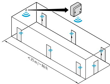
AH30 (RS485 Hub) - Placement of the Hub, 1-16 doors
