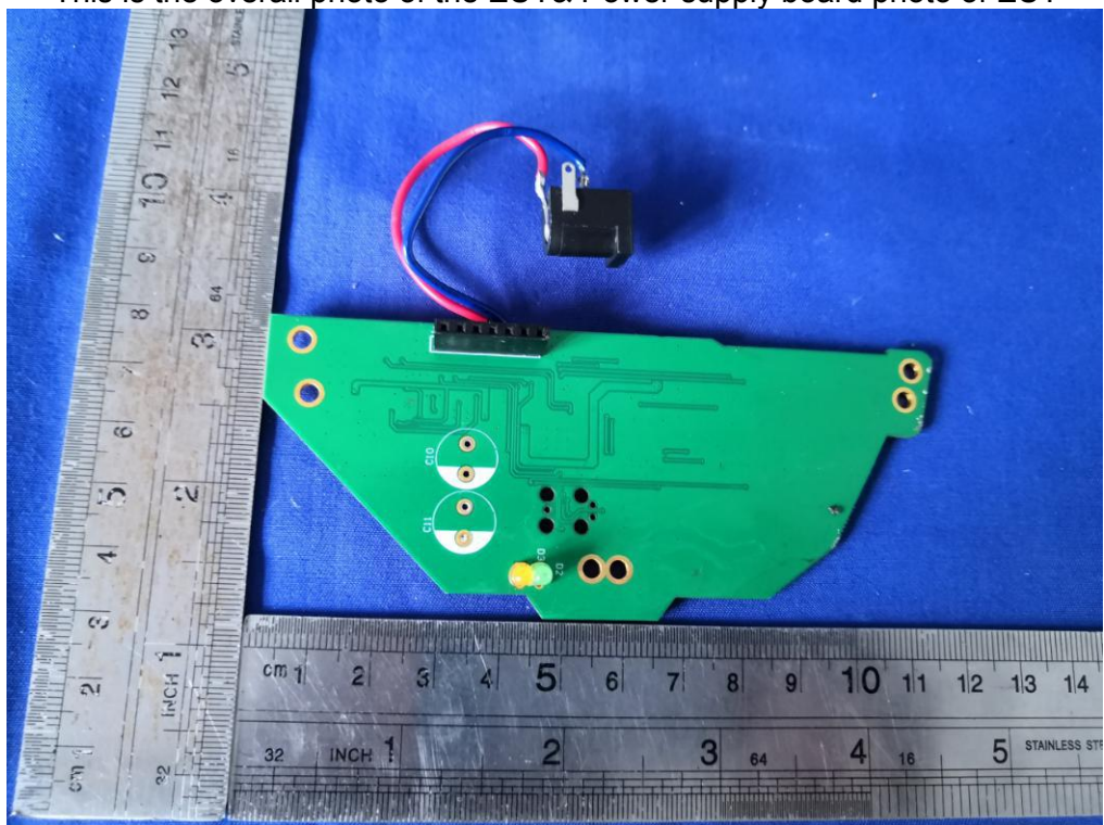
This is the overall photo of the EUT& Power supply board photo of EUT
