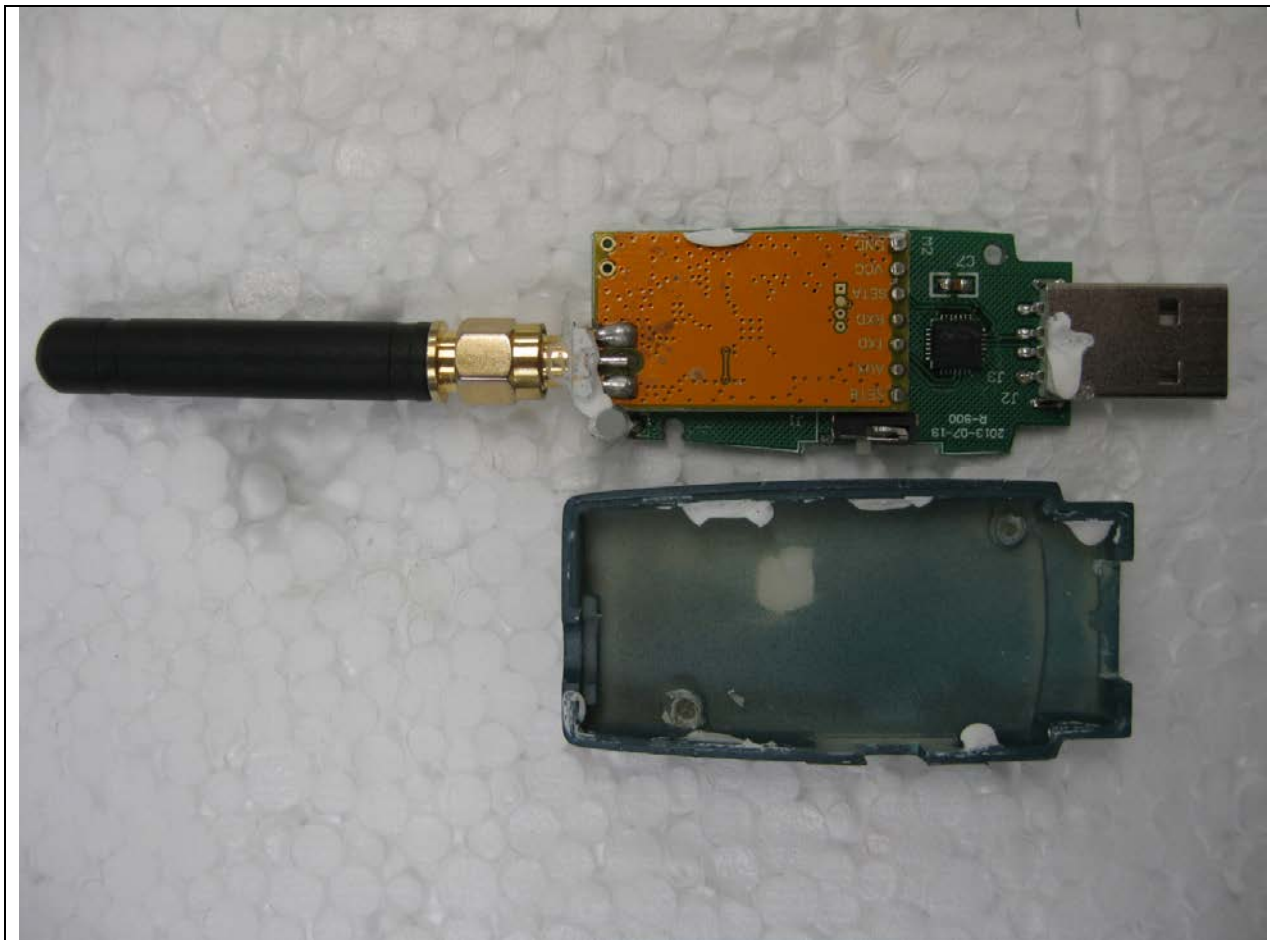
RF Adapter – PCB Removed from Enclosure
