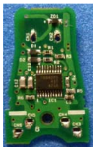
Printed Circuit Board Front View
