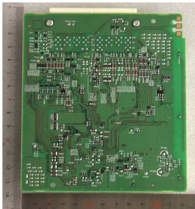
Antenna side
