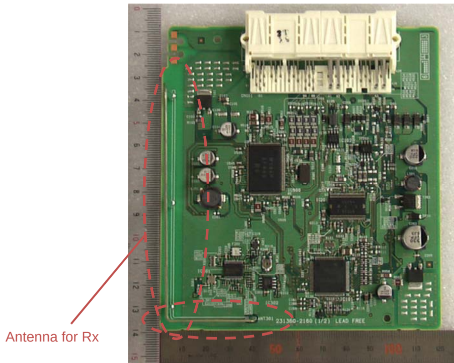
Component side
