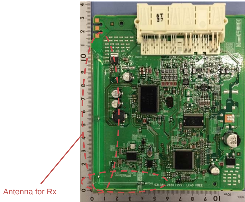
Component side
