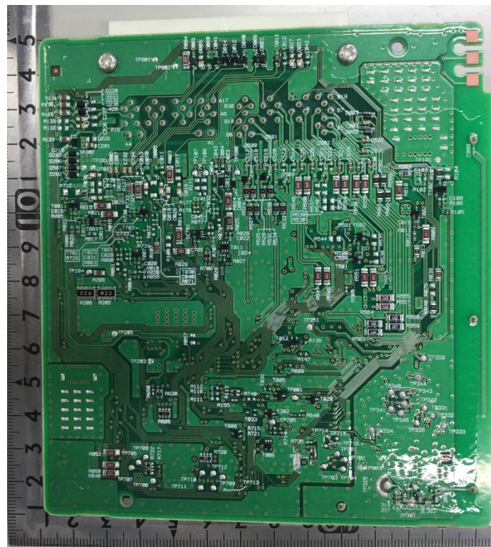
Antenna side
