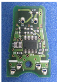
Front (PCB)
