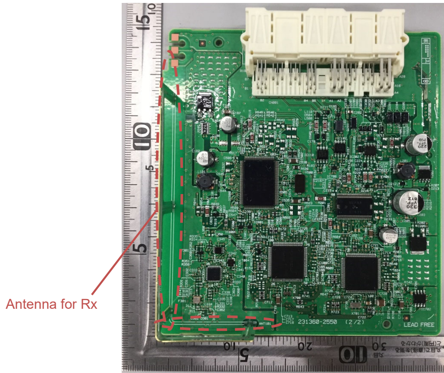
Component side
