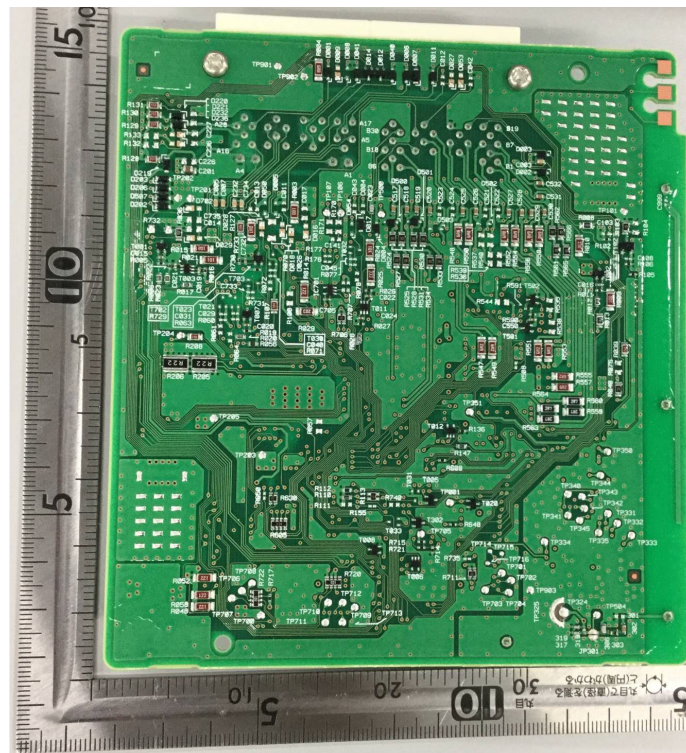
Antenna side
