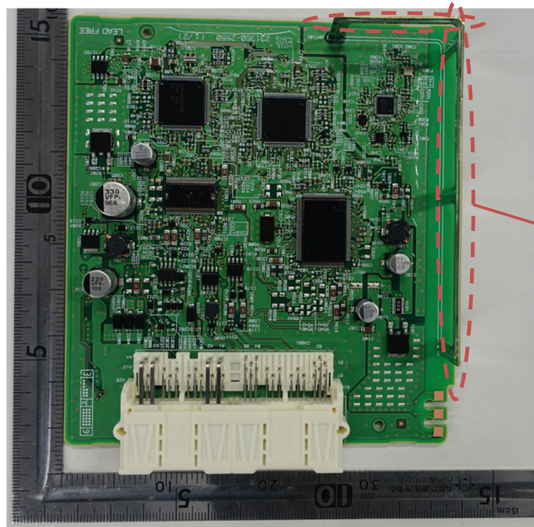
Component side
