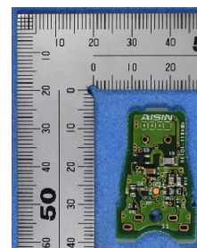
Rear (PCB)
