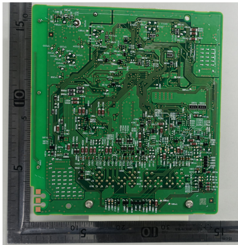
Antenna side
