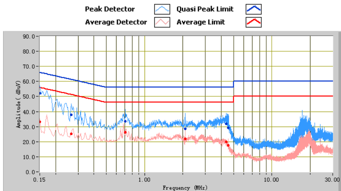
Phase Neutral Plot 120V
