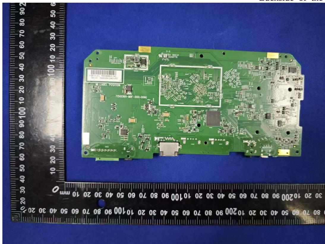
Figure 26 Backside of the Main Board
