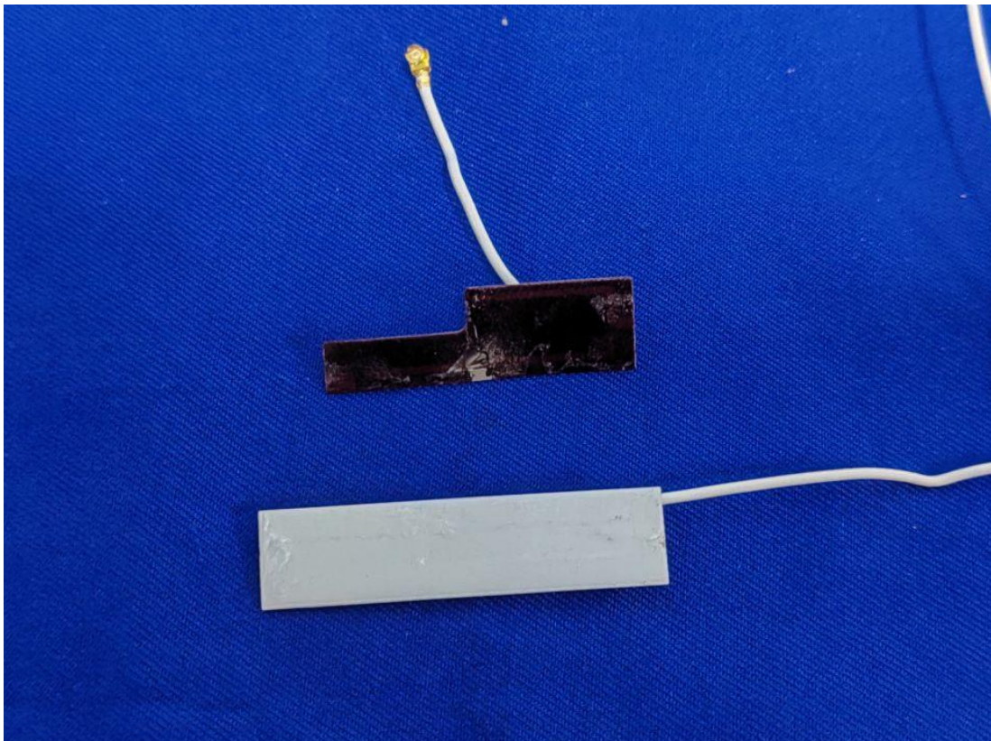
Figure 30 Frontside of the WIFI and NFC
