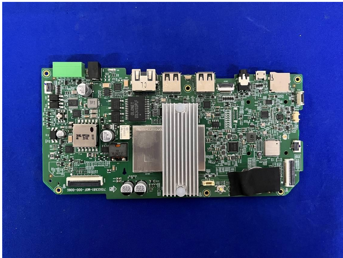
Figure 23 Frontside of the Main Board
