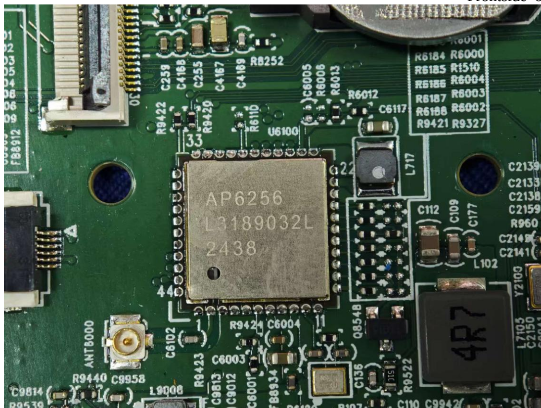
Figure 33 Frontside of the WIFI
