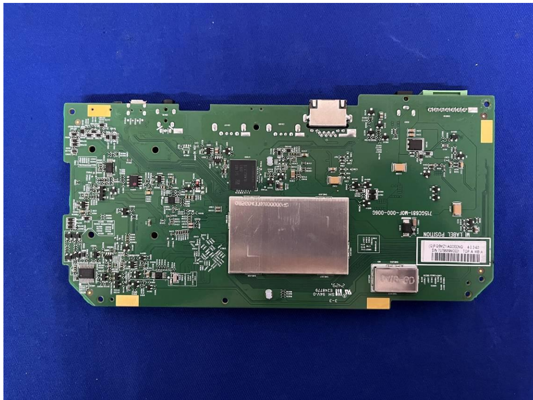
Figure 25 Backside of the Main Board
