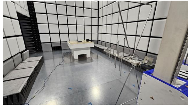
Set-up photo for radiated tests below 1 GHz photo
