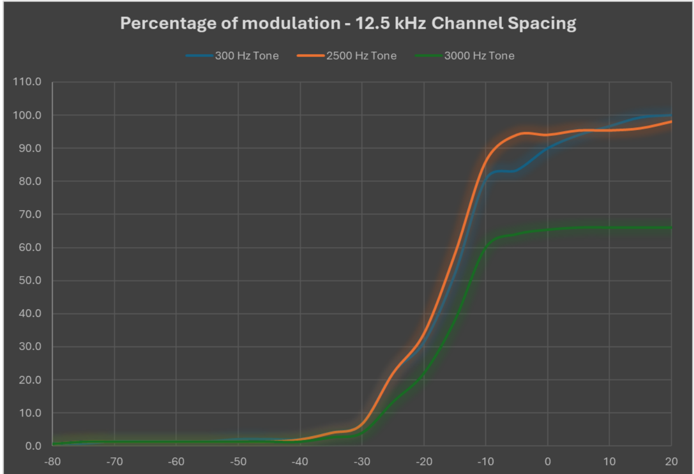
Modulation Limiting at 74.0 MHz (12.5 kHz)
