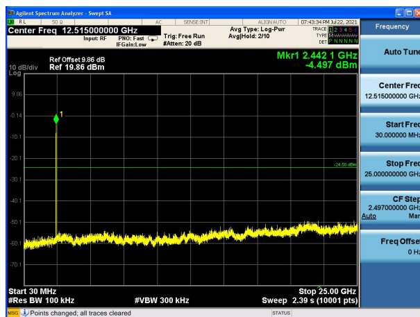
CH39(Hopping off)
