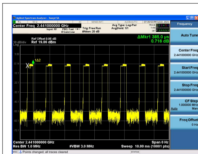
Modulation: \pi/4 DQPSK 2DH1 2441
