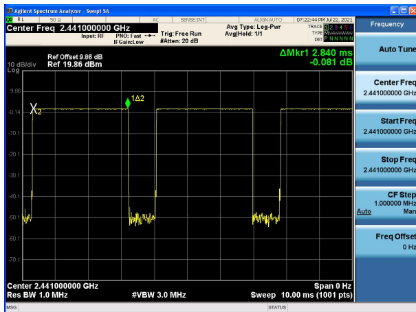
Modulation: GFSK DH5 2441
