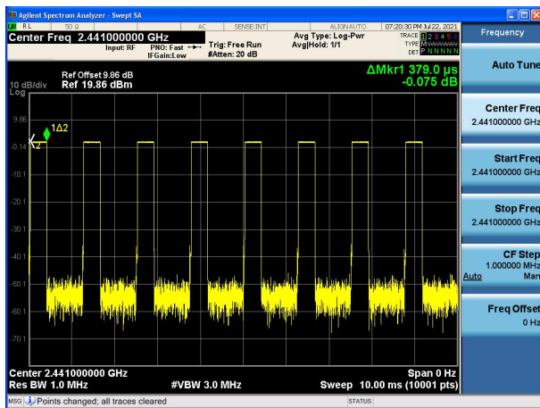
Modulation: GFSK DH1 2441
