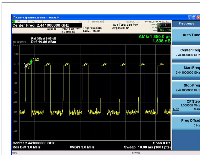
Modulation: 8DPSK 3DH1 2441
