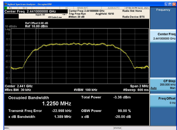
Modulation: 8DPSK 2441MHz
