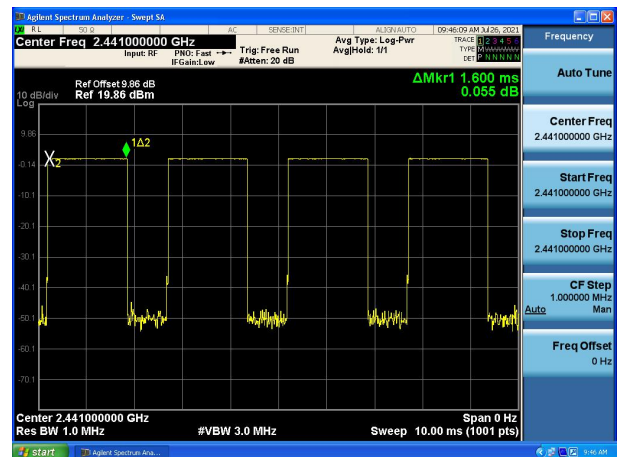
Modulation: GFSK DH3 2441
