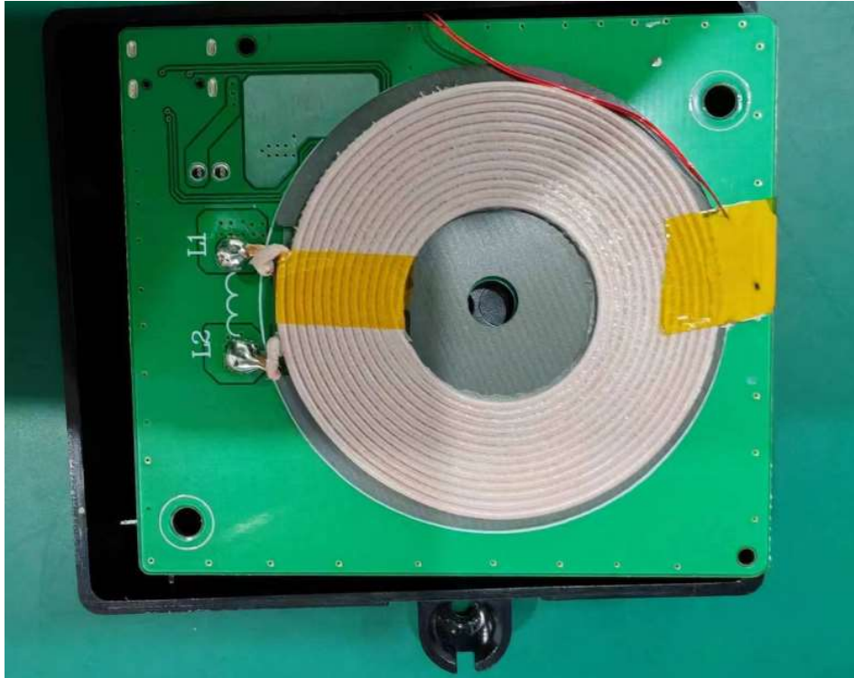
Antenna coil
