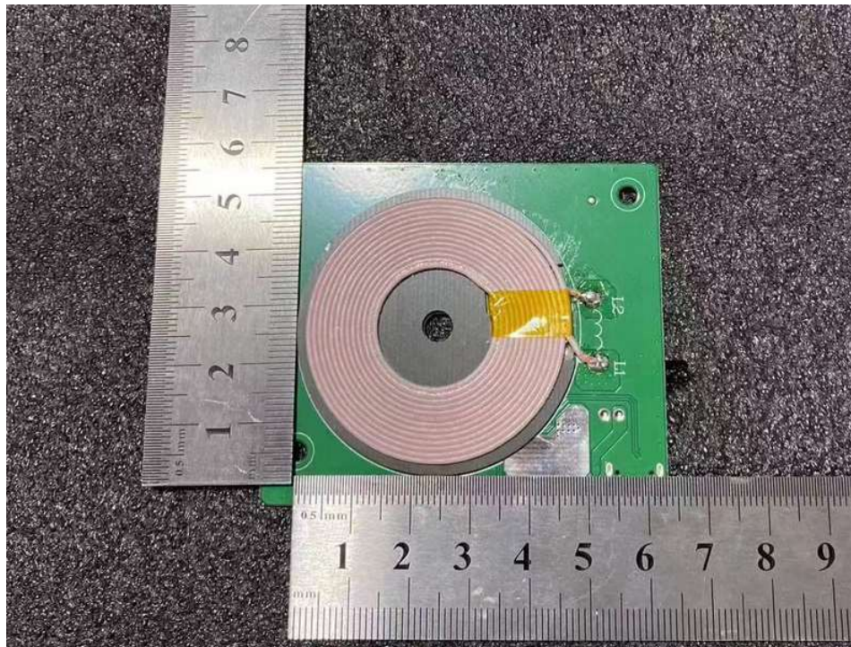
Antenna coil
