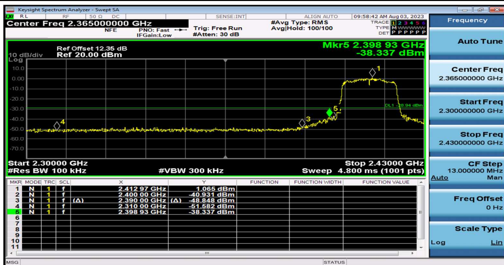
11N20SISO_Ant1_Low_2412
