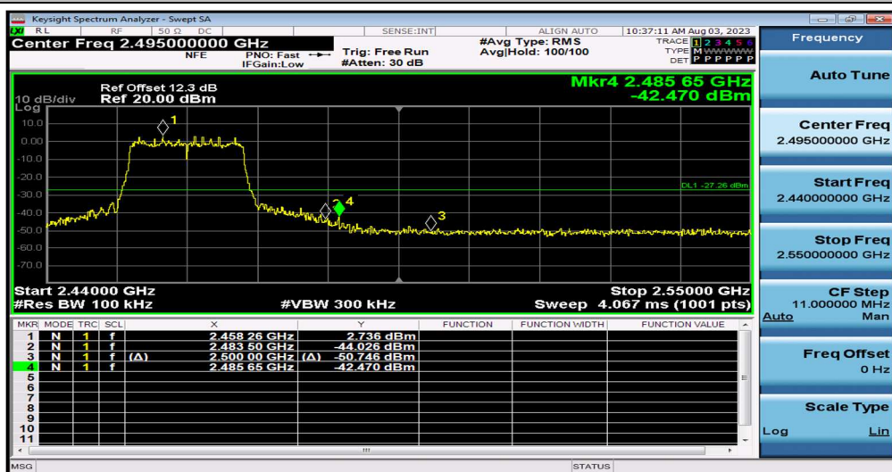
11N20SISO_Ant1_High_2462
