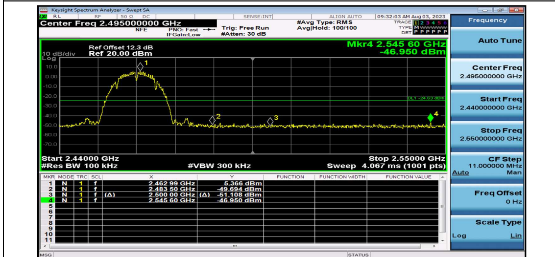
11B_Ant1_High_2462
