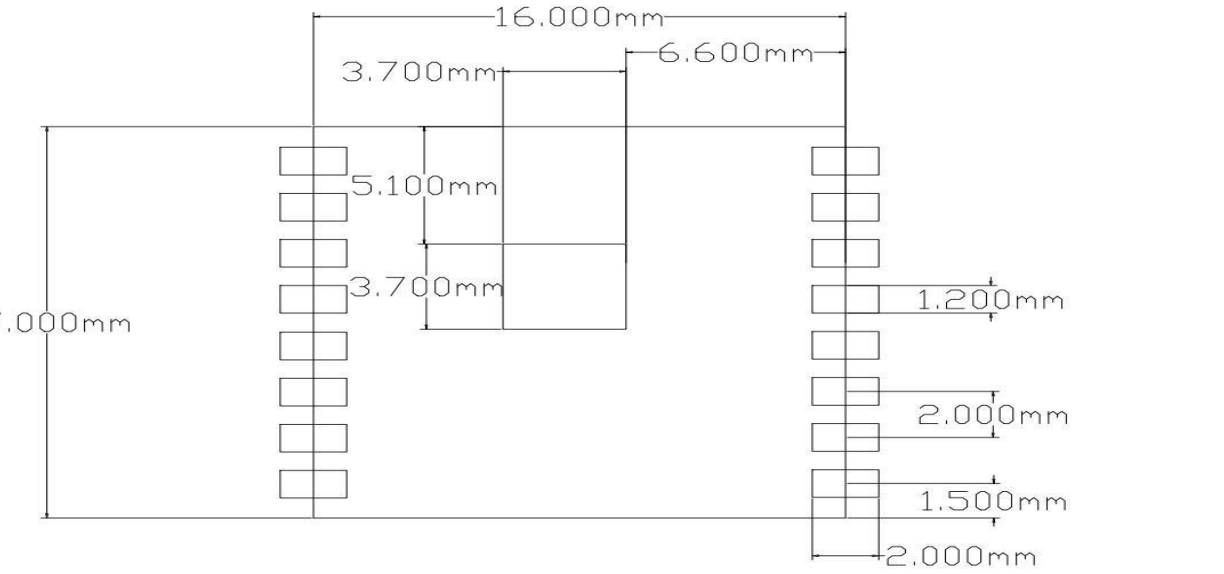
Figure 9 Recommended PCB Packaging Dimensions
