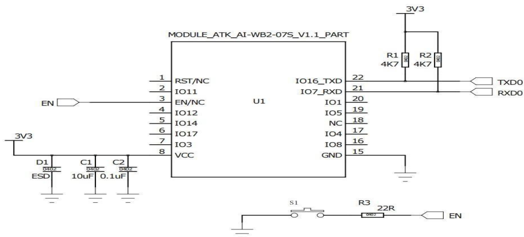
Figure 8 Application Guidance Circuit
