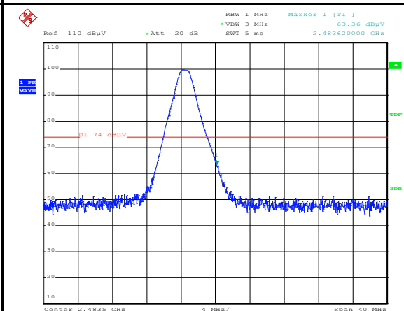
Band Edge, Right Side (Peak - Horizontal)
