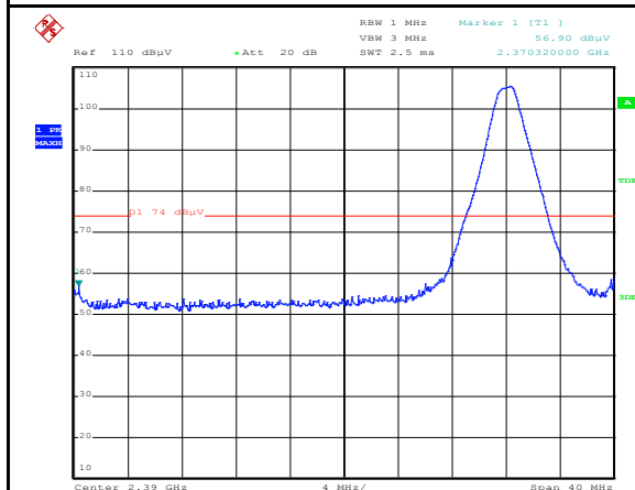
Band Edge, Left Side (Peak - Horizontal)
