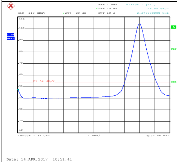
Band Edge, Left Side (Average - Vertical)
