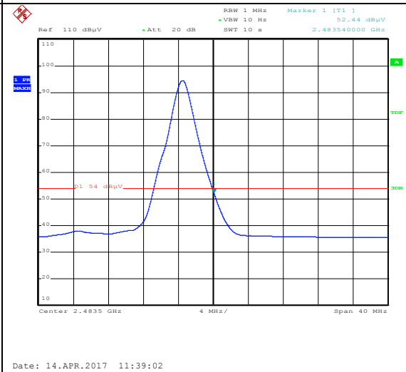
Band Edge, Right Side (Average - Vertical)
