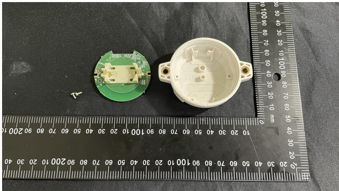
BL1 (Without Temperature Sensor)
