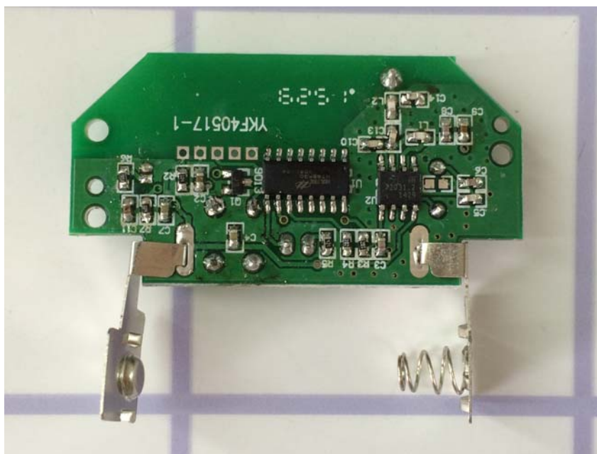
PCB 1 side 2
