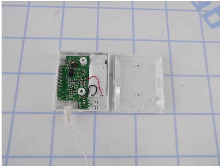
Internal view 2
