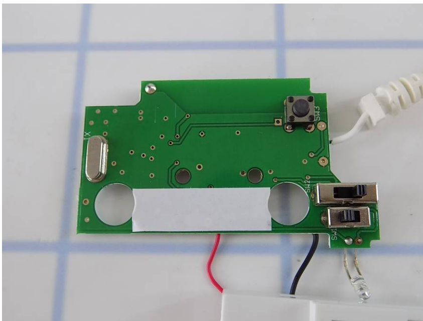
PCB side 2
