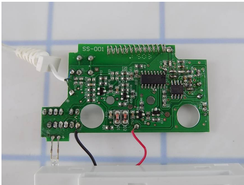
PCB side1
