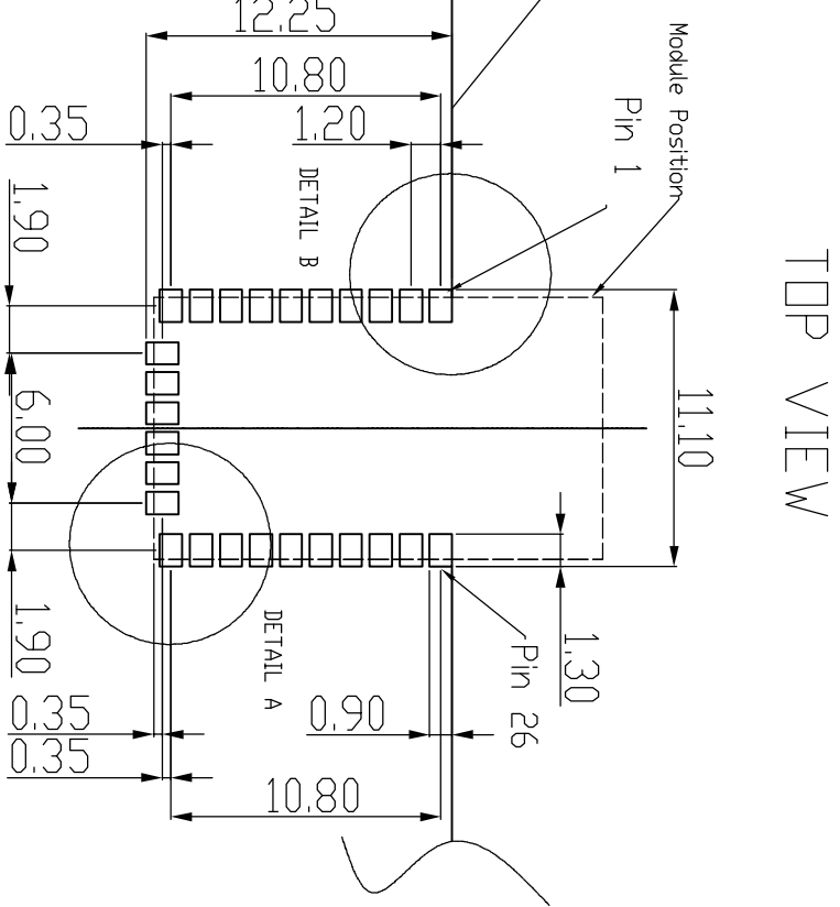
RECOMMENDED P.C.B PATTERN LAYOUT
