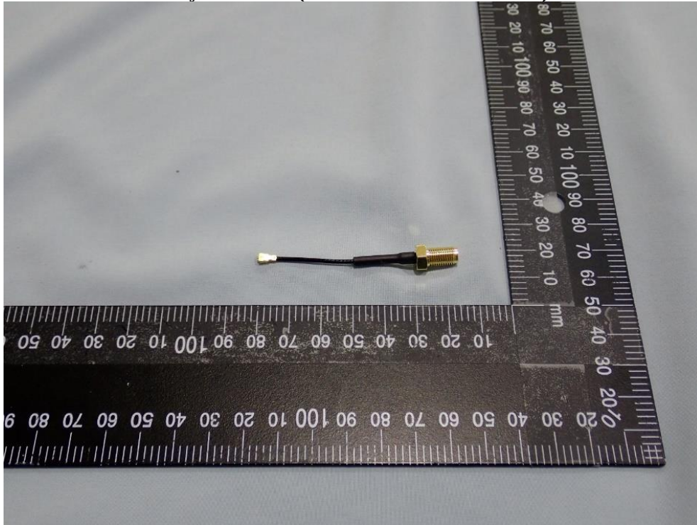
Accessory: Antenna(RFDPA171300SBLB801) Pic 3
