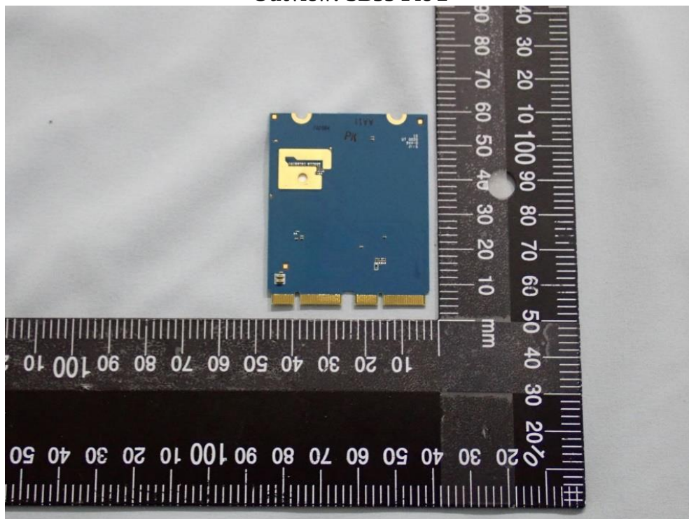
Outview: SB35 Pic 2
