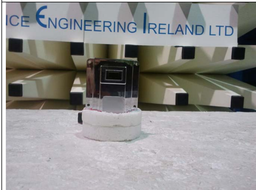
Fig 2 Test setup
