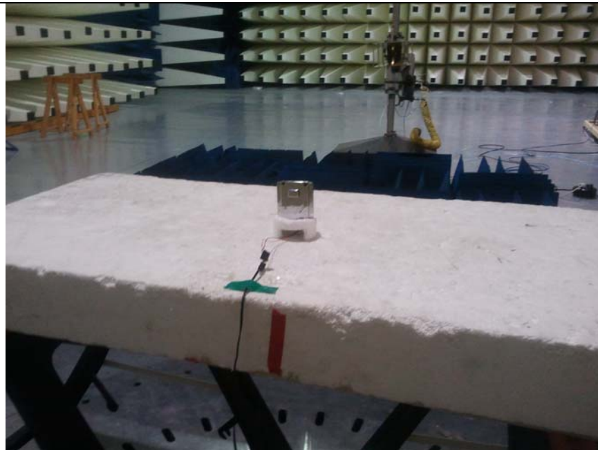
Fig 5 Test setup
