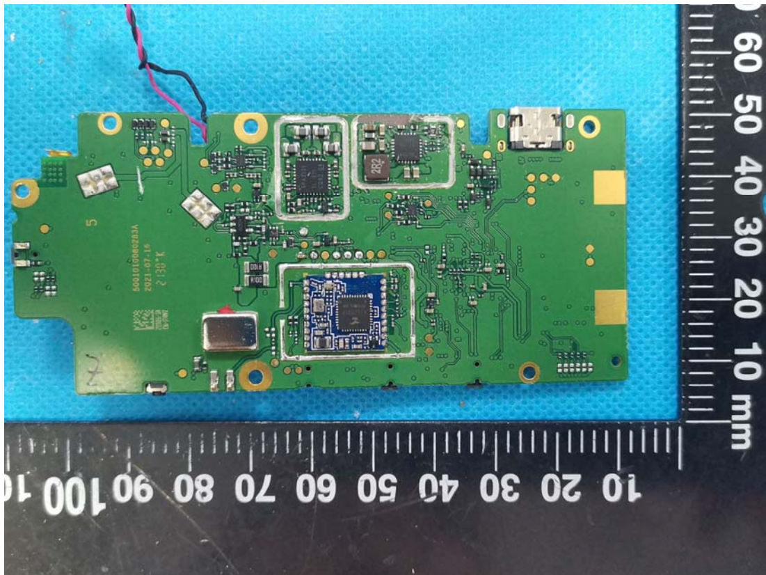
Bluetooth Chip
