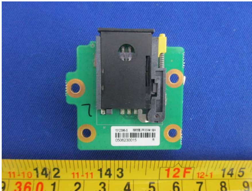
EUT – PCB Board 2 Top View
