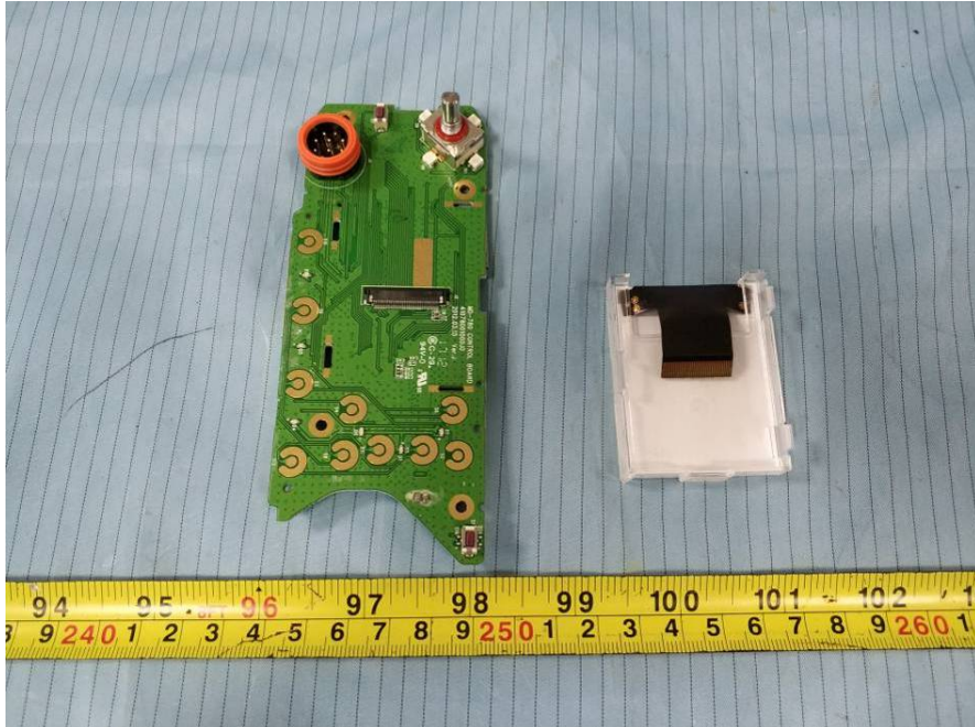
RF unit – Cover off View 3
