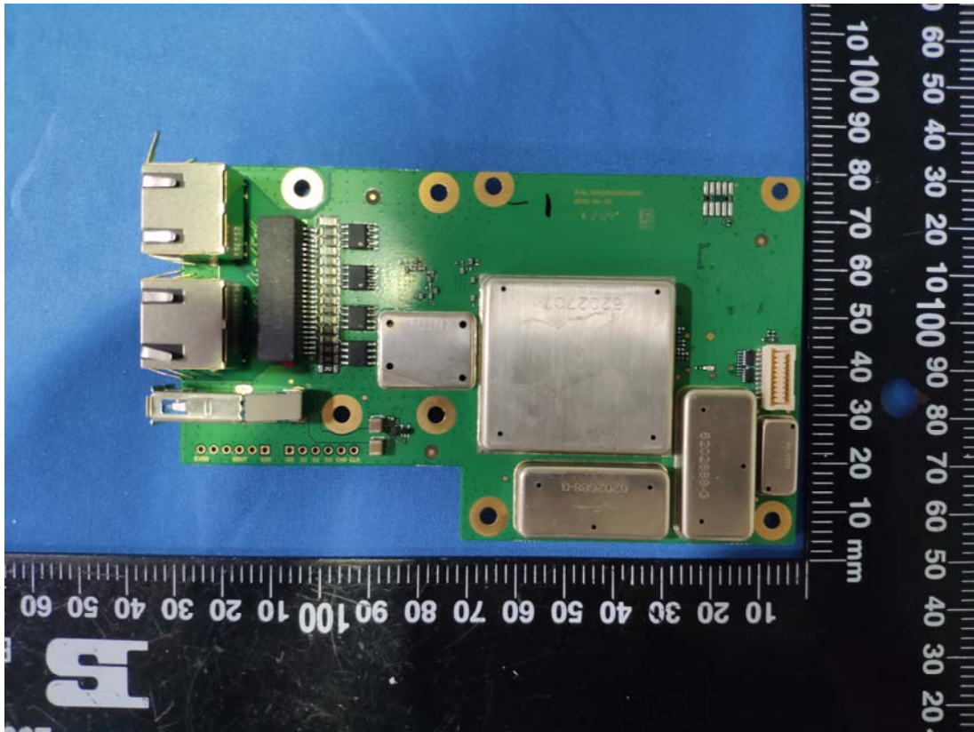
Network Board (Double Ethernet Interface Configuration)
