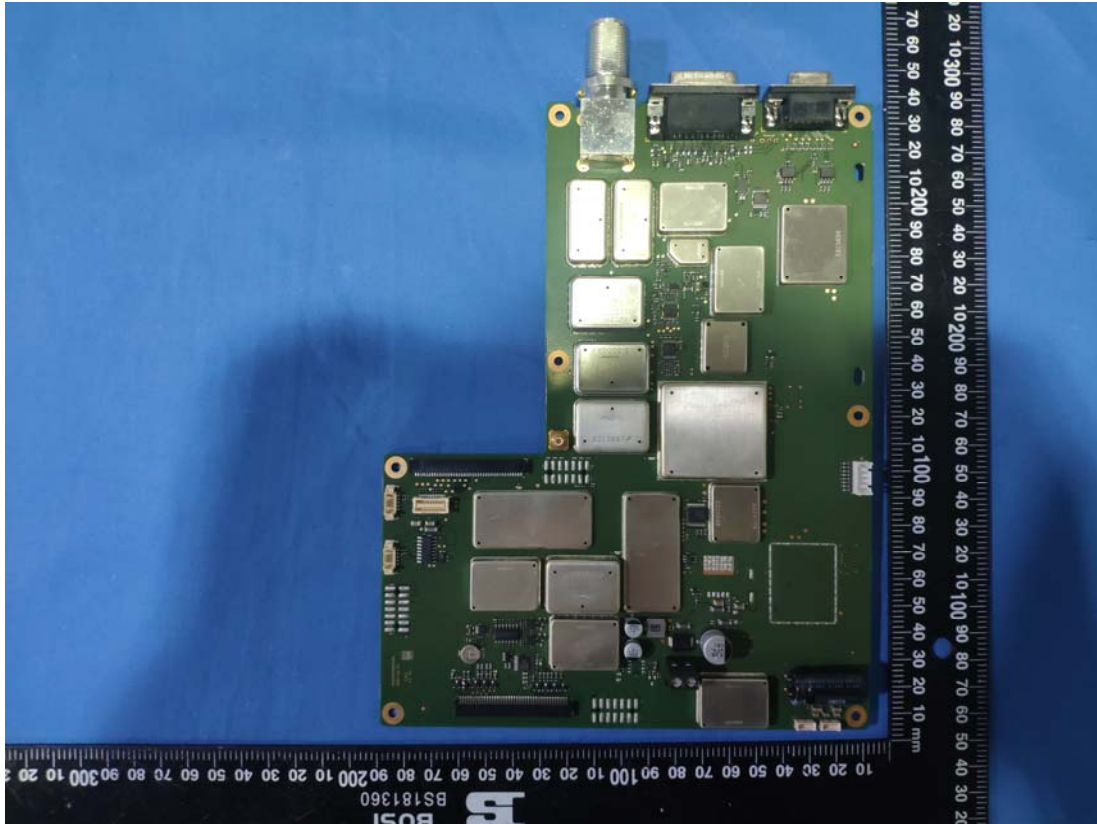
Main Board
