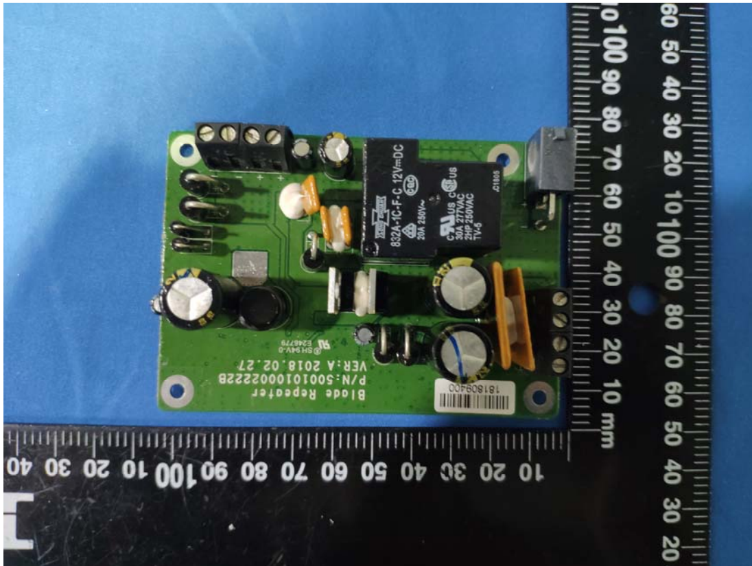
Float Charging Board
