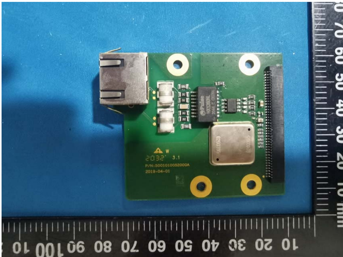
Network Board (Single Ethernet Interface Configuration)
