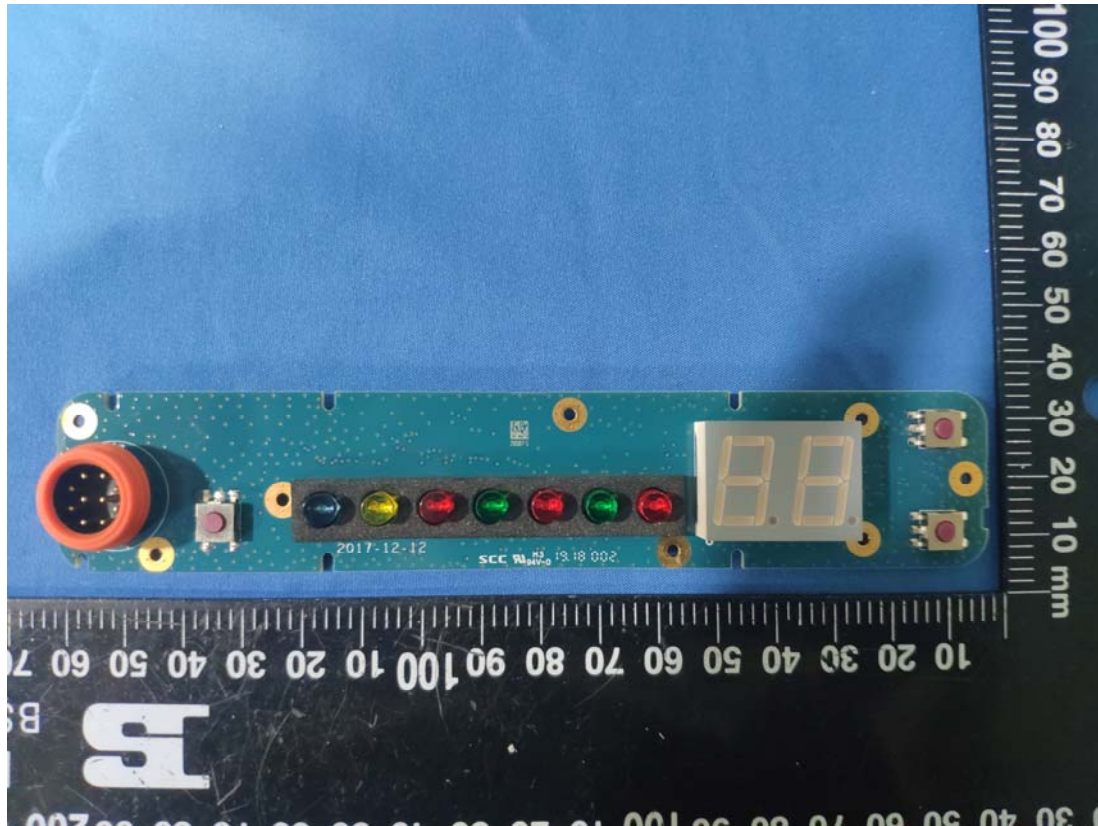
Control Panel
