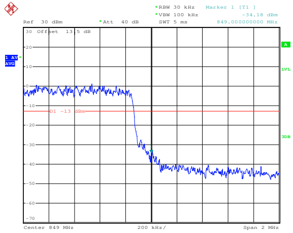
16QAM High channel-15 RB offset 0
