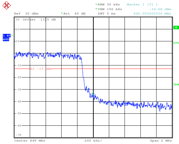
QPSK High channel-15 RB offset 0
