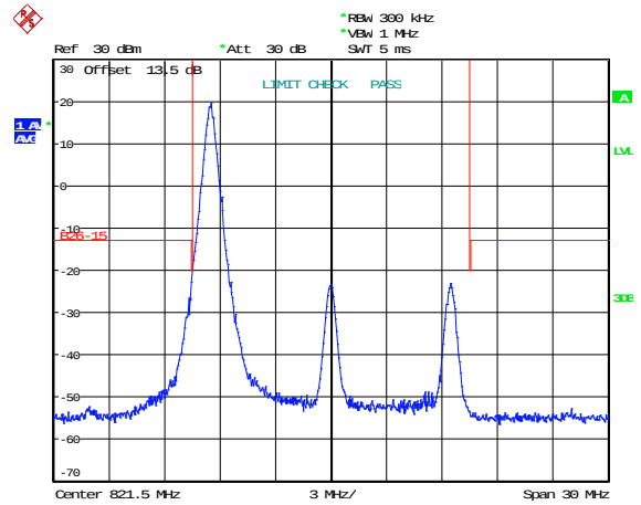
16QAM Low channel-36 RB offset 0
