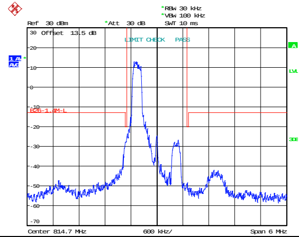
16QAM Low channel-6 RB offset 0
