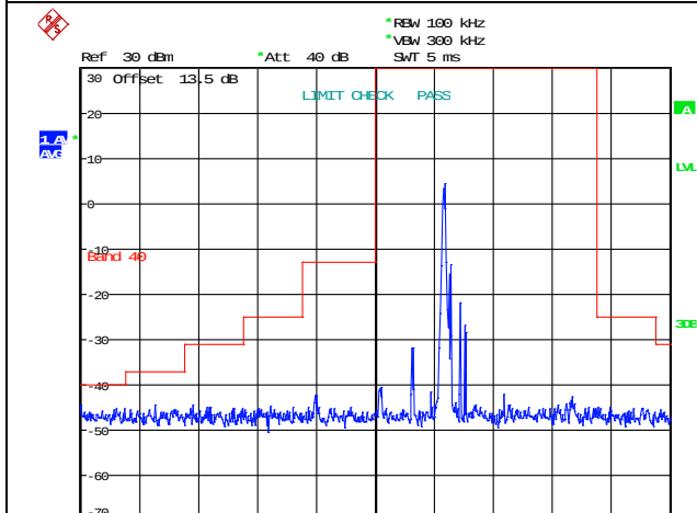
QPSK Low channel-1 RB offset max
