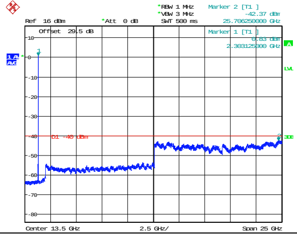
QPSK Middle channel-1GHz~25GHz
