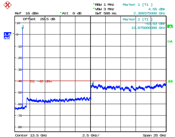
QPSK High channel-1GHz~25GHz
