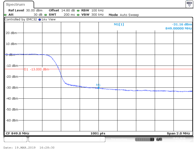
LTE FDD Band 26(824MHz-849MHz), Nominal Bandwidth: 15MHz
