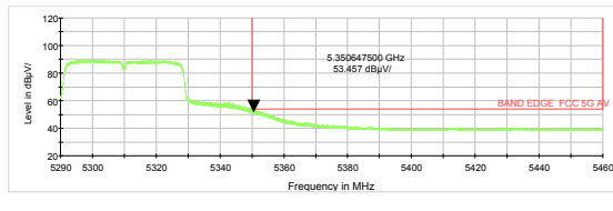
802.11n HT40-Channel 62: Average
