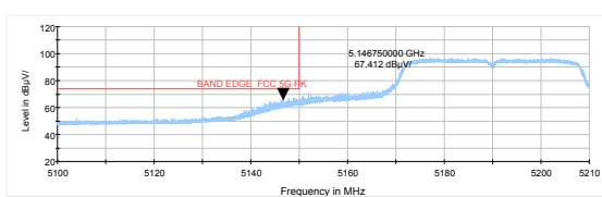
802.11n HT40-Channel 38: Peak
