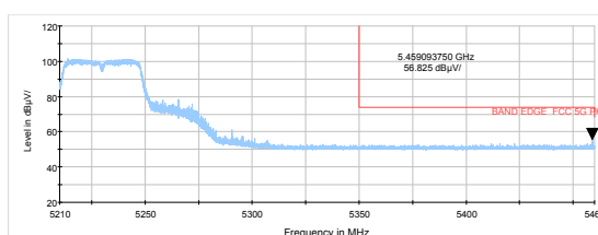
802.11n HT40-Channel 46: Average
