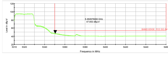
802.11n HT20-Channel 64: Average
