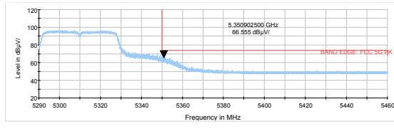
802.11n HT40-Channel 62: Peak
