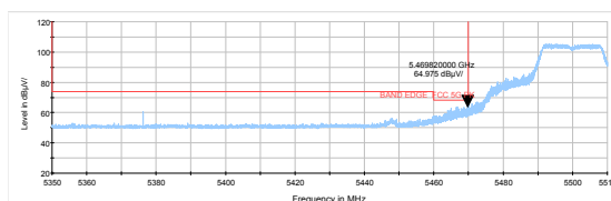
802.11n HT20-Channel 100: Peak
