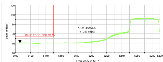
802.11n HT40-Channel 54: Average
