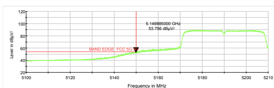
802.11n HT40-Channel 38: Average
