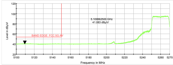
802.11n HT40-Channel 54: Peak
