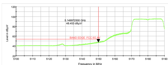
802.11n HT20-Channel 36: Average
