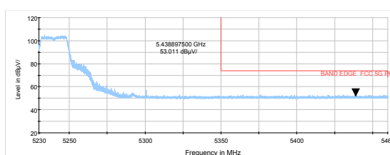
802.11n HT20-Channel 48: Average
