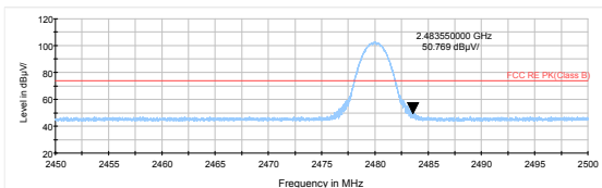
3DH5-Channel 78: Peak
