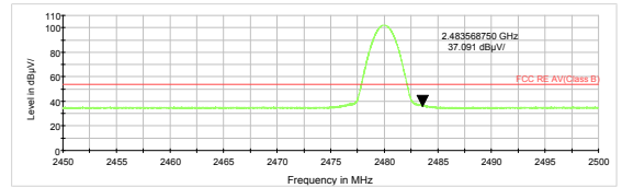
DH5-Channel 78: Average
