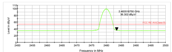
3DH5-Channel 78: Average
