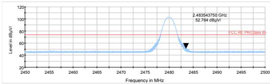
DH5-Channel 78: Peak
