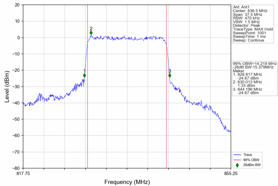
n5_15kHz_SISO_NTNV_15MHz_CP-OFDM_16_QAM_836.5MHz_Outer_Full
