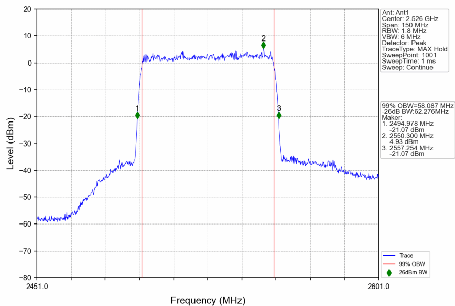
n41_30kHz_SISO_NTNV_60MHz_DFT-s-OFDM_64_QAM_2526MHz_Outer_Full
