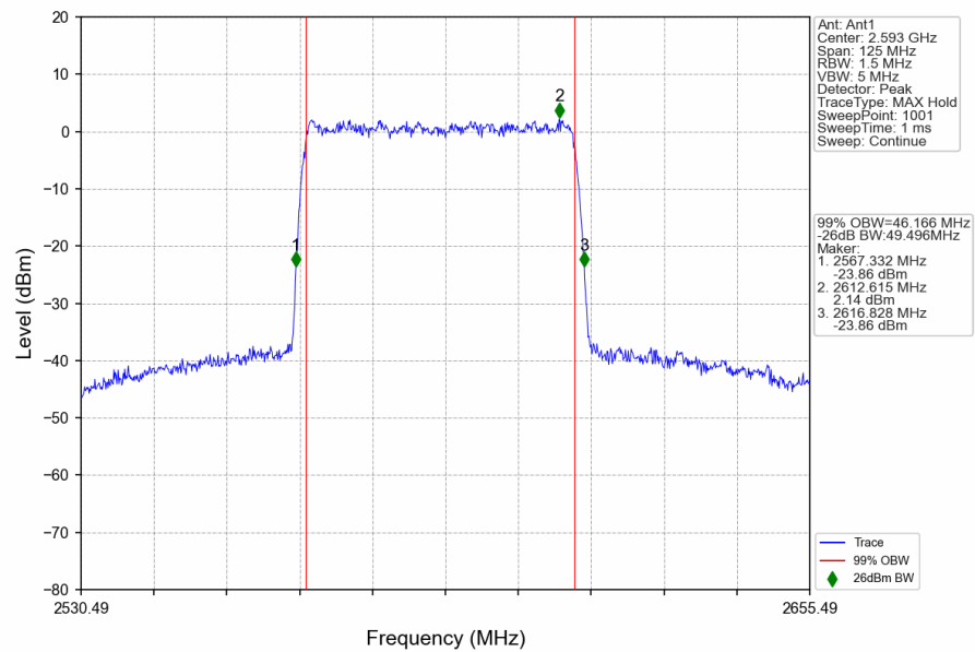
n41_30kHz_SISO_NTNV_50MHz_DFT-s-OFDM_256_QAM_2592.99MHz_Outer_Full
