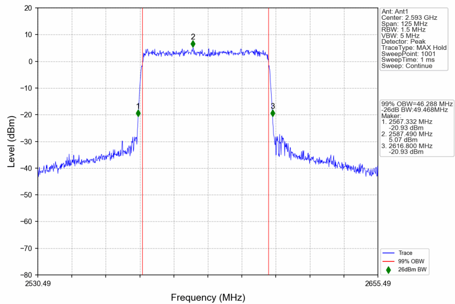
n41_30kHz_SISO_NTNV_50MHz_DFT-s-OFDM_16_QAM_2592.99MHz_Outer_Full
