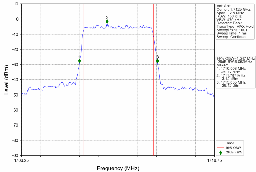
n66_15kHz_SISO_NTNV_5MHz_DFT-s-OFDM_64_QAM_1712.5MHz_Outer_Full
