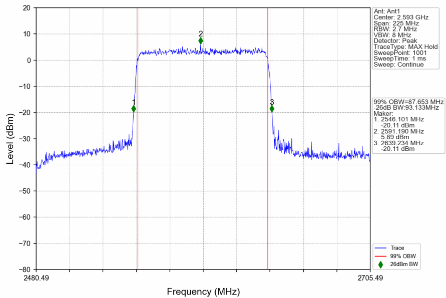
n41_30kHz_SISO_NTNV_90MHz_DFT-s-OFDM_16_QAM_2592.99MHz_Outer_Full
