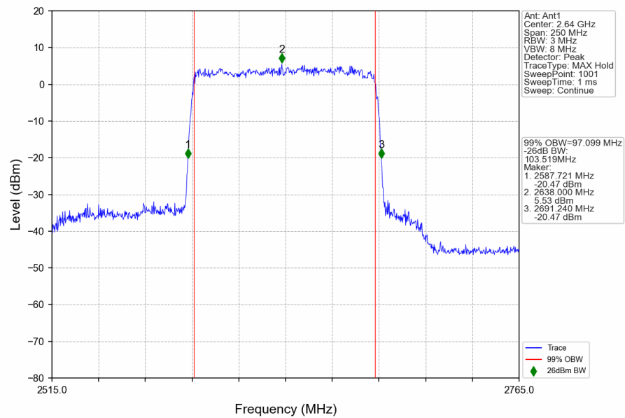
n41_30kHz_SISO_NTNV_100MHz_DFT-s-OFDM_64_QAM_2640MHz_Outer_Full
