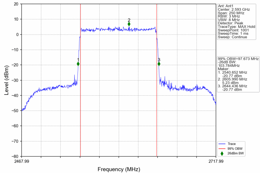
n41_30kHz_SISO_NTNV_100MHz_DFT-s-OFDM_16_QAM_2592.99MHz_Outer_Full
