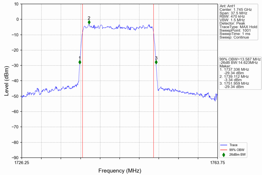
n66_15kHz_SISO_NTNV_15MHz_DFT-s-OFDM_256_QAM_1745MHz_Outer_Full
