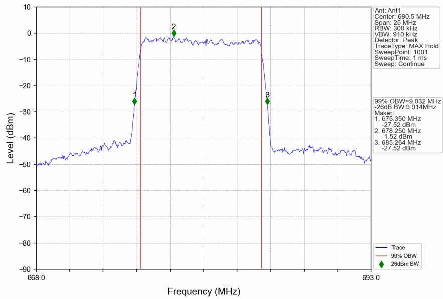
n71_15kHz_SISO_NTNV_10MHz_DFT-s-OFDM 256 QAM_680.5MHz_Outer_Full
