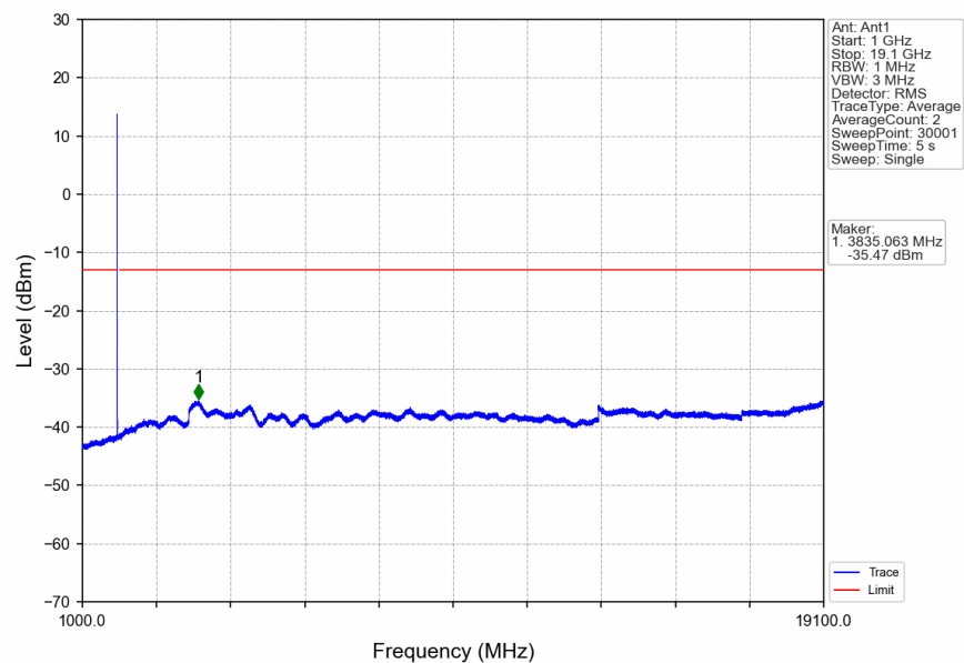
n2_15kHz_SISO_NTNV_5MHz_CP-OFDM_QPSK_1852.5MHz_Edge_1RB_Left
