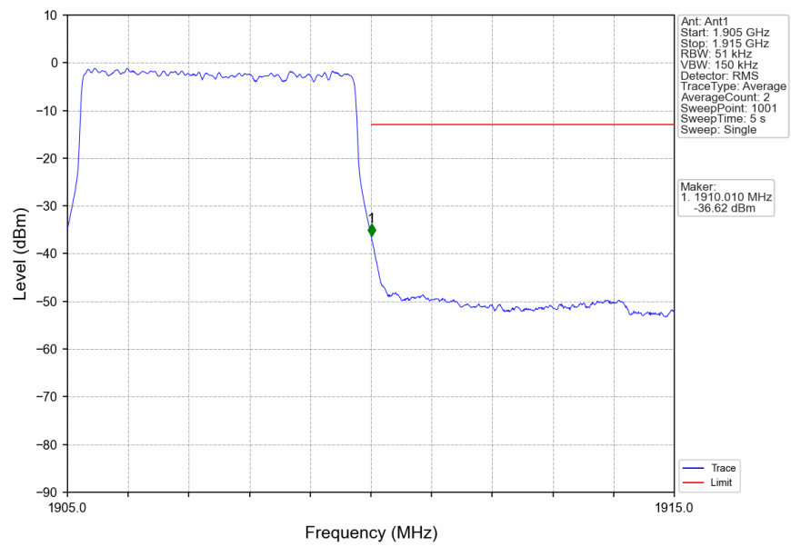
n2_15kHz_SISO_NTNV_5MHz_DFT-s-OFDM_QPSK_1907.5MHz_Outer_Full
