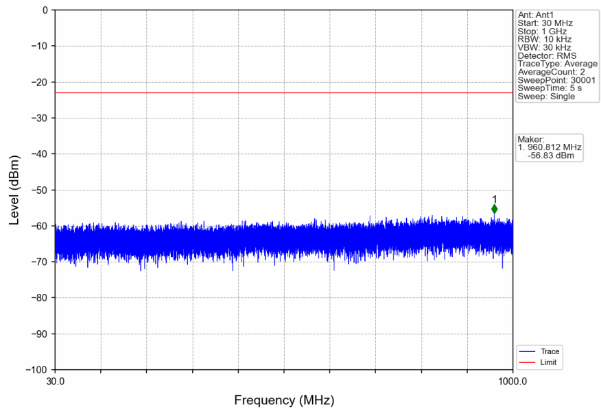
n2_15kHz_SISO_NTNV_5MHz_DFT-s-OFDM_QPSK_1907.5MHz_Inner_1RB_Right
