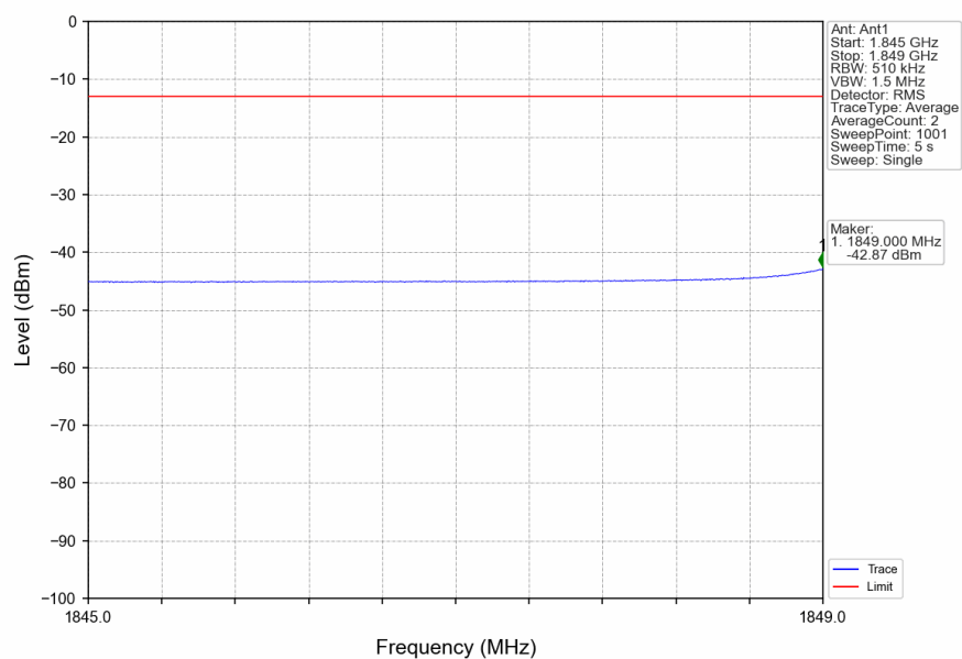
n2_15kHz_SISO_NTNV_5MHz_DFT-s-OFDM_QPSK_1852.5MHz_Edge_1RB_Left
