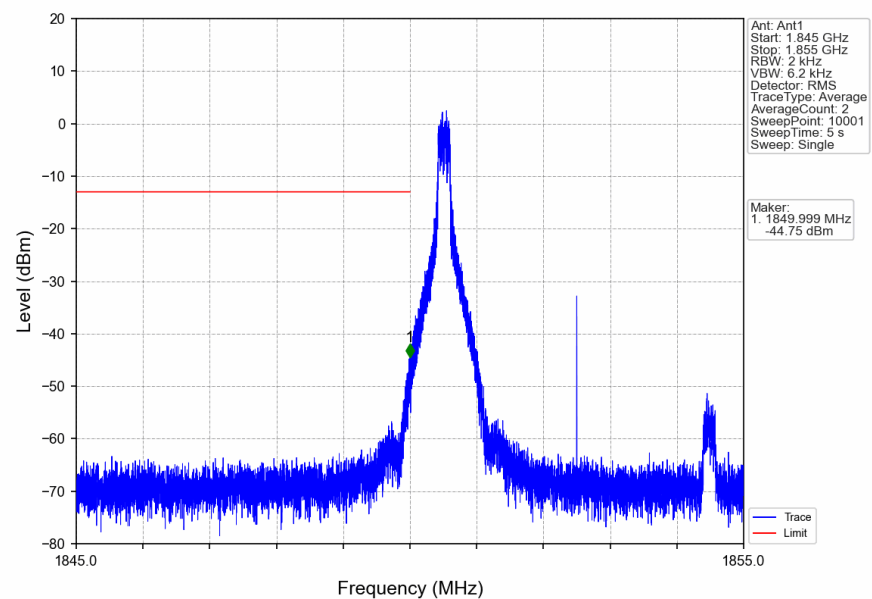
n2_15kHz_SISO_NTNV_5MHz_DFT-s-OFDM_QPSK_1852.5MHz_Inner_1RB_Left
