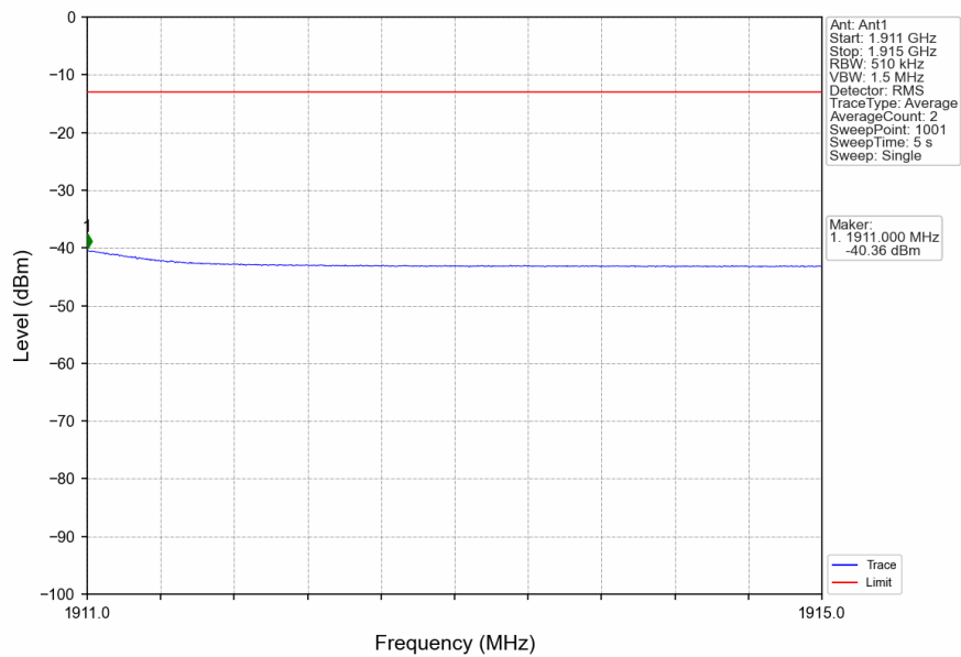
n2_15kHz_SISO_NTNV_5MHz_DFT-s-OFDM PI/2 BPSK_1907.5MHz_Edge_1RB_Right
