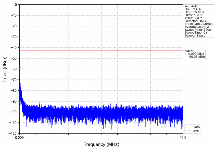
n2_15kHz_SISO_NTNV_5MHz_DFT-s-OFDM QPSK_1852.5MHz_Edge_1RB_Left
