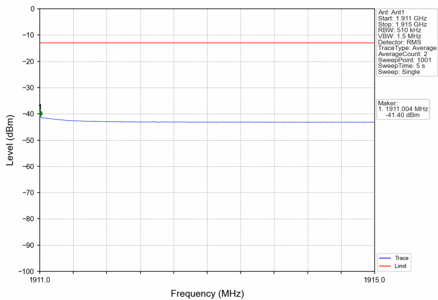
n2_15kHz_SISO_NTNV_5MHz_DFT-s-OFDM PI/2 BPSK_1907.5MHz_Inner_1RB_Right
