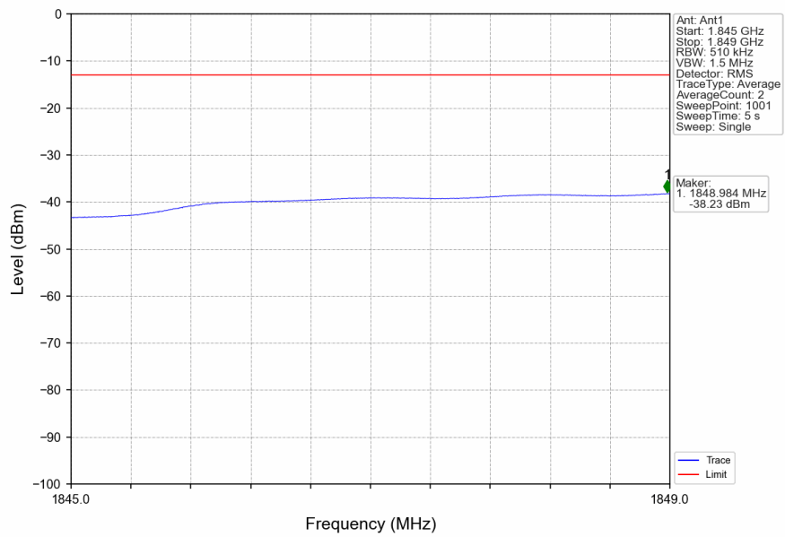
n2_15kHz_SISO_NTNV_5MHz_DFT-s-OFDM_QPSK_1852.5MHz_Outer_Full
