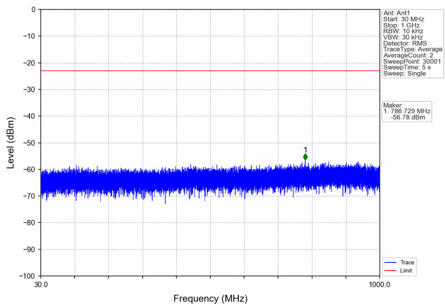
n2_15kHz_SISO_NTNV_5MHz_DFT-s-OFDM_QPSK_1852.5MHz_Inner_1RB_Left
