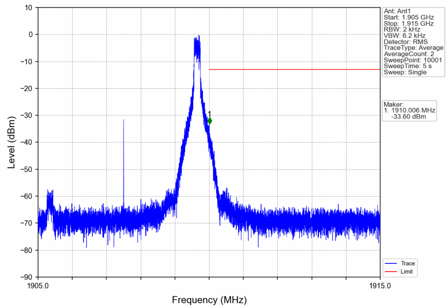
n2_15kHz_SISO_NTNV_5MHz_CP-OFDM_QPSK_1907.5MHz_Edge_1RB_Right
