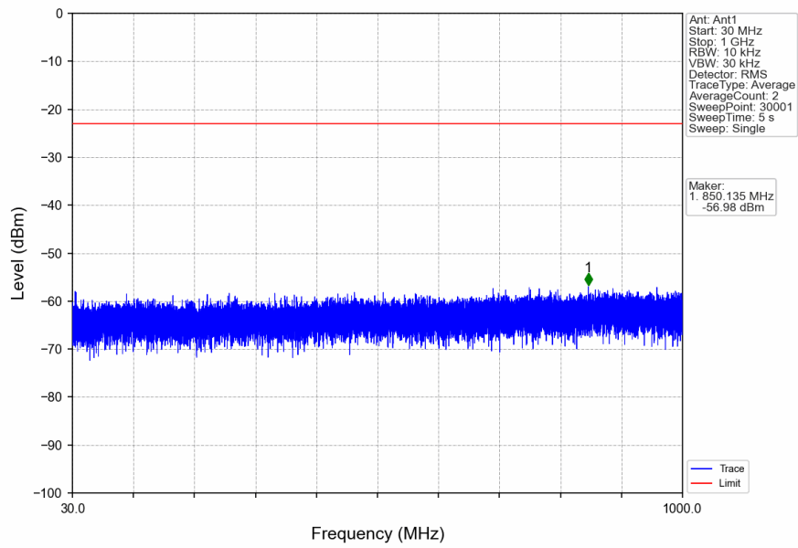
n2_15kHz_SISO_NTNV_5MHz_DFT-s-OFDM_QPSK_1907.5MHz_Edge_1RB_Right
