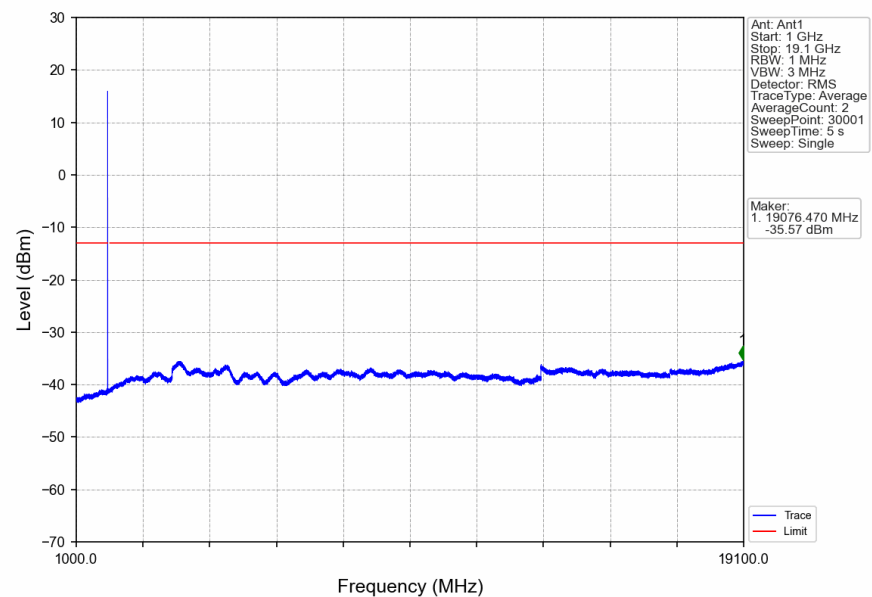
n2_15kHz_SISO_NTNV_5MHz_DFT-s-OFDM_QPSK_1852.5MHz_Inner_1RB_Left
