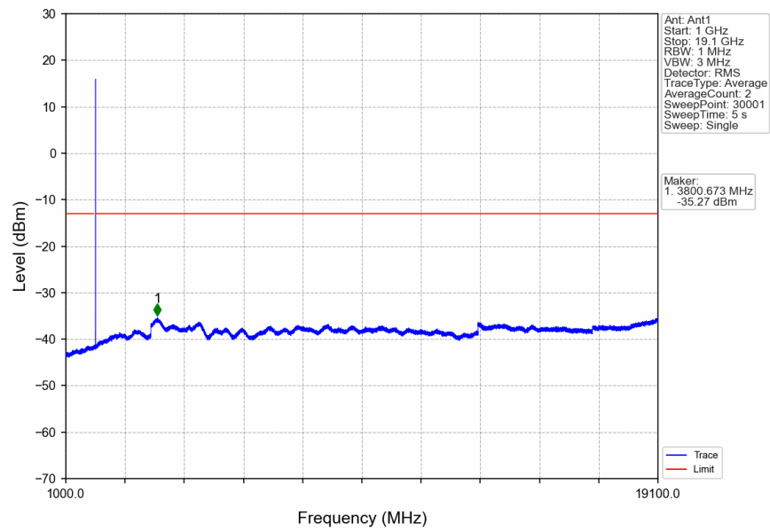
n2_15kHz_SISO_NTNV_5MHz_DFT-s-OFDM_QPSK_1907.5MHz_Edge_1RB_Right
