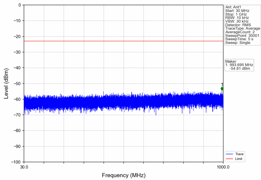
n2_15kHz_SISO_NTNV_5MHz_DFT-s-OFDM PI/2 BPSK_1907.5MHz_Outer_Full
