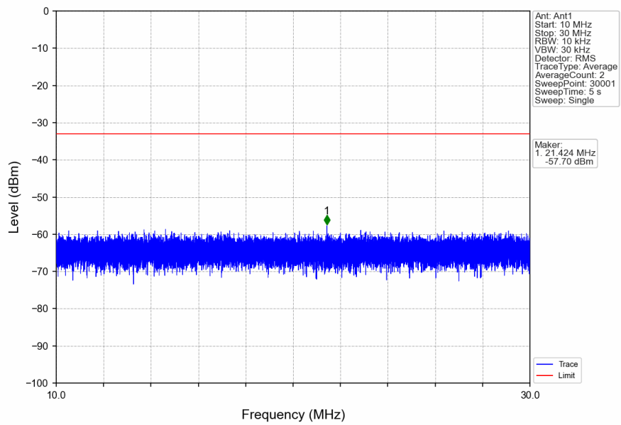
n2_15kHz_SISO_NTNV_5MHz_DFT-s-OFDM QPSK_1907.5MHz_Edge_1RB_Right
