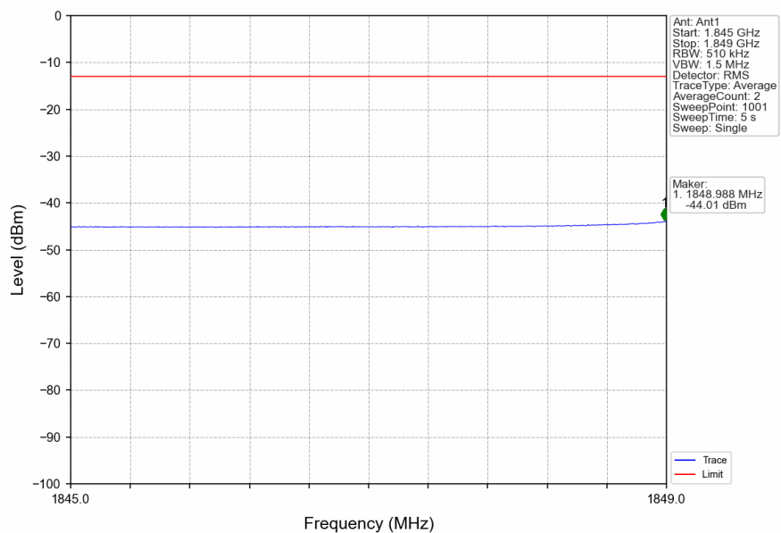
n2_15kHz_SISO_NTNV_5MHz_DFT-s-OFDM_QPSK_1852.5MHz_Inner_1RB_Left
