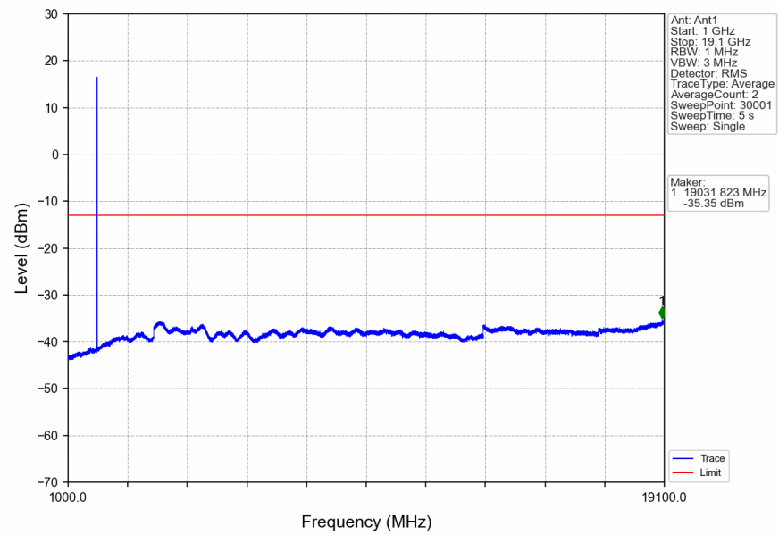
n2_15kHz_SISO_NTNV_5MHz_DFT-s-OFDM_QPSK_1880MHz_Edge_1RB_Left
