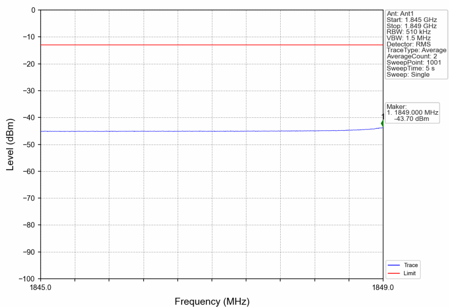
n2_15kHz_SISO_NTNV_5MHz_CP-OFDM_QPSK_1852.5MHz_Edge_1RB_Left
