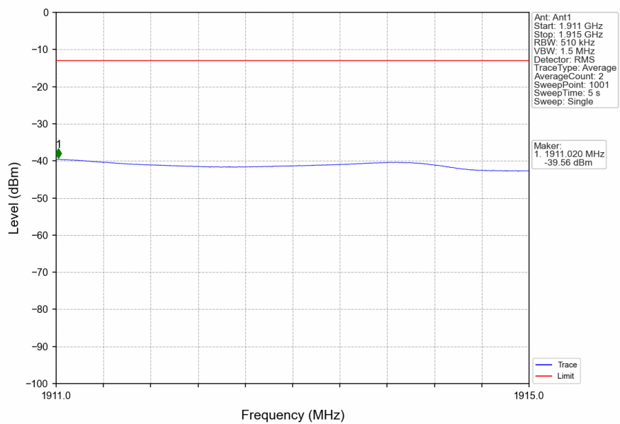
n2_15kHz_SISO_NTNV_5MHz_DFT-s-OFDM_QPSK_1907.5MHz_Outer_Full
