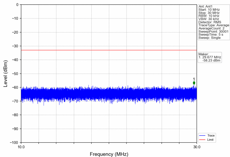
n2_15kHz_SISO_NTNV_5MHz_DFT-s-OFDM_QPSK_1907.5MHz_Inner_1RB_Right
