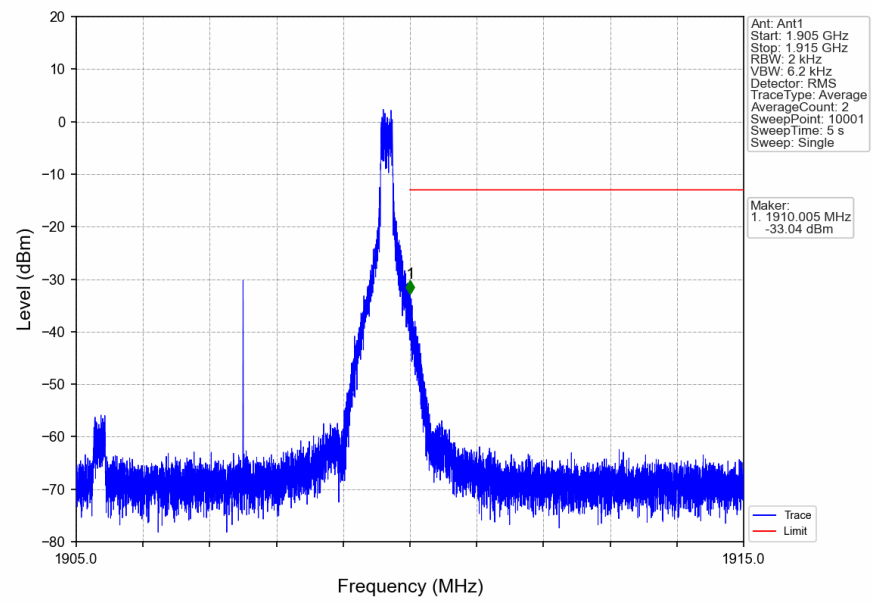
n2_15kHz_SISO_NTNV_5MHz_DFT-s-OFDM QPSK_1907.5MHz_Edge_1RB_Right
