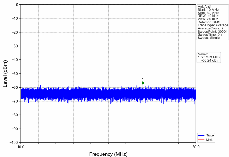
n2_15kHz_SISO_NTNV_5MHz_DFT-s-OFDM QPSK_1852.5MHz_Edge_1RB_Left
