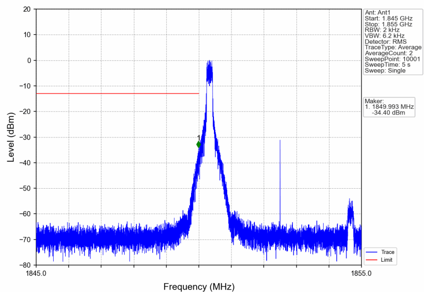
n2_15kHz_SISO_NTNV_5MHz_CP-OFDM_QPSK_1852.5MHz_Edge_1RB_Left
