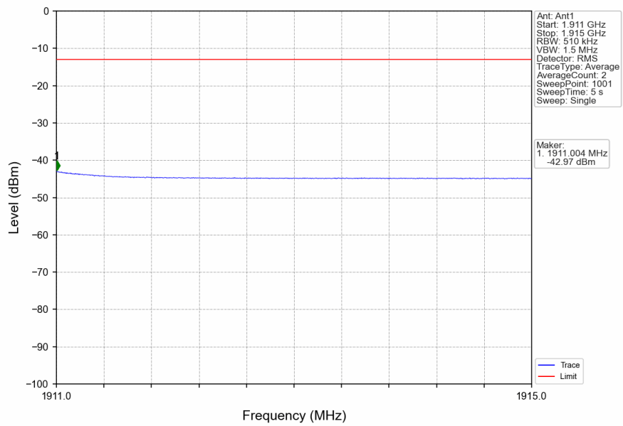
n2_15kHz_SISO_NTNV_5MHz_CP-OFDM_QPSK_1907.5MHz_Edge_1RB_Right
