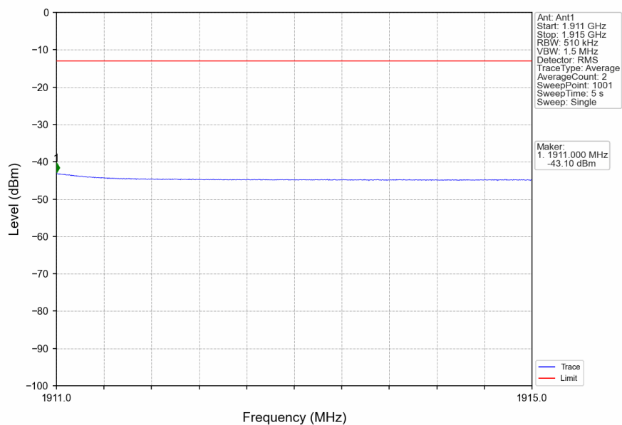
n2_15kHz_SISO_NTNV_5MHz_DFT-s-OFDM_QPSK_1907.5MHz_Inner_1RB_Right
