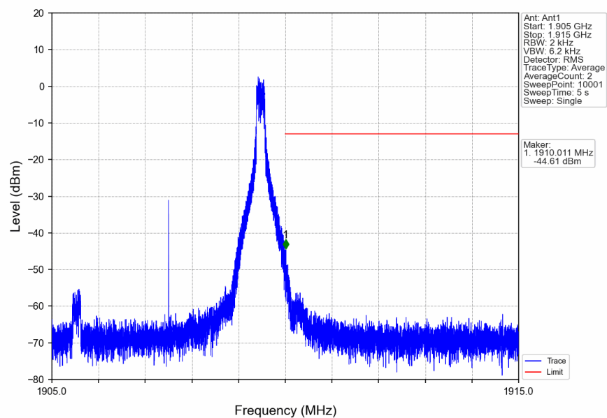
n2_15kHz_SISO_NTNV_5MHz_DFT-s-OFDM_QPSK_1907.5MHz_Inner_1RB_Right
