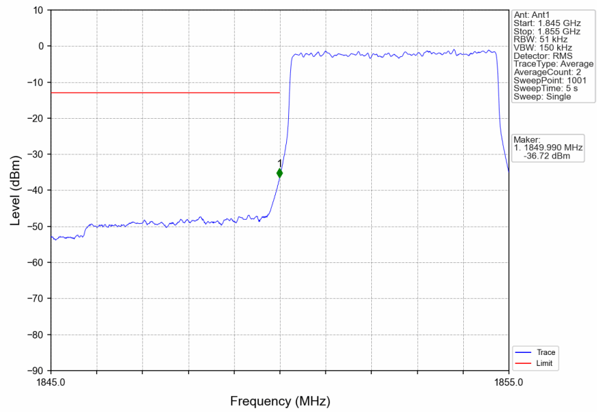
n2_15kHz_SISO_NTNV_5MHz_DFT-s-OFDM_QPSK_1852.5MHz_Outer_Full
