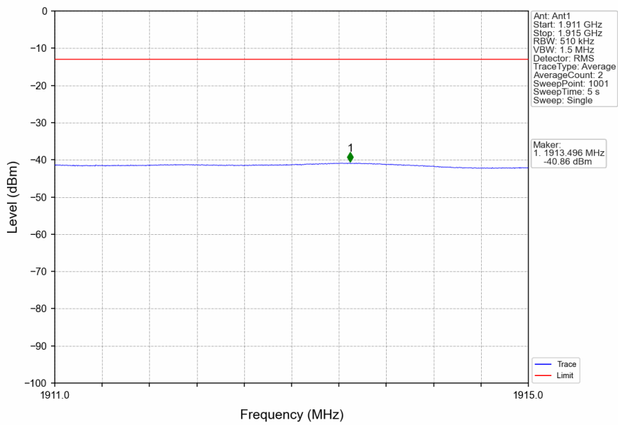
n2_15kHz_SISO_NTNV_10MHz_DFT-s-OFDM_PI/2_BPSK_1905MHz_Outer_Full
