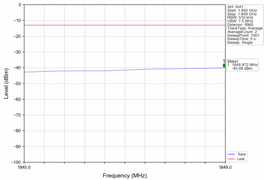
n2_15kHz_SISO_NTNV_10MHz_DFT-s-OFDM_QPSK_1855MHz_Outer_Full
