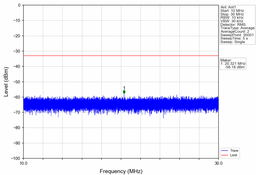
n2_15kHz_SISO_NTNV_10MHz_DFT-s-OFDM_QPSK_1880MHz_Edge_1RB_Left
