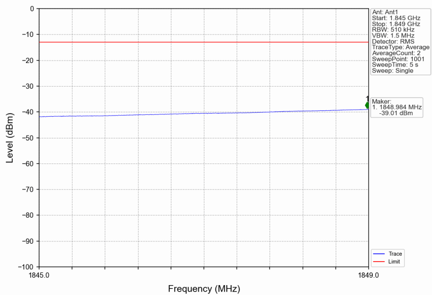
n2_15kHz_SISO_NTNV_10MHz_CP-OFDM QPSK_1855MHz_Outer_Full
