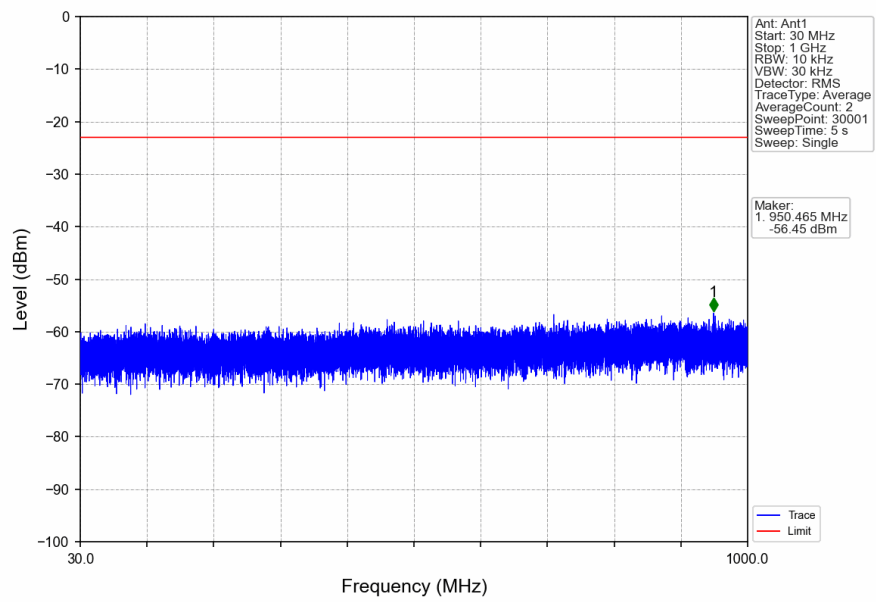
n2_15kHz_SISO_NTNV_10MHz_DFT-s-OFDM_QPSK_1905MHz_Inner_1RB_Right
