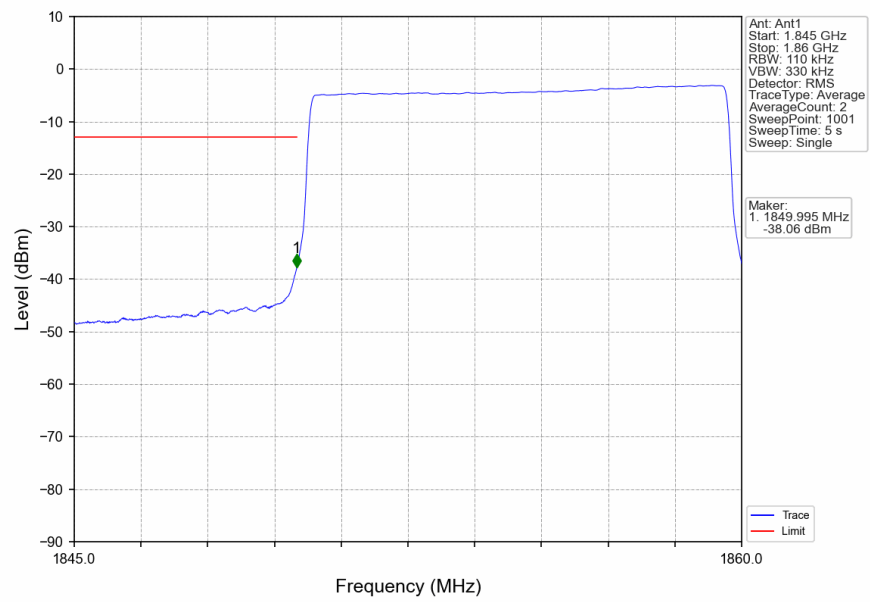
n2_15kHz_SISO_NTNV_10MHz_CP-OFDM QPSK_1855MHz_Outer_Full
