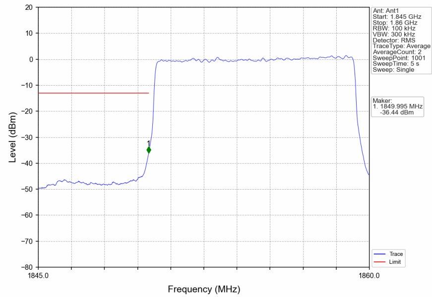
n2_15kHz_SISO_NTNV_10MHz_DFT-s-OFDM_PI/2_BPSK_1855MHz_Outer_Full
