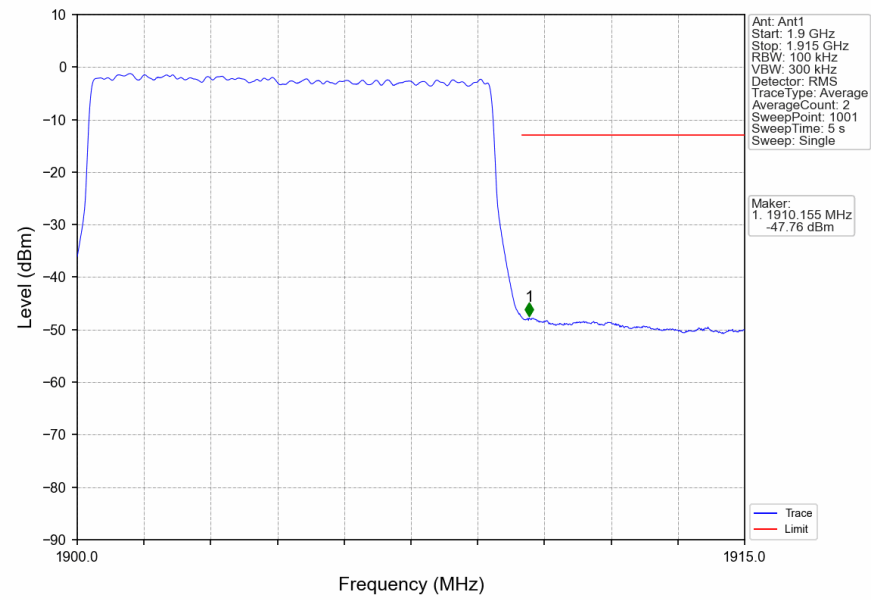
n2_15kHz_SISO_NTNV_10MHz_DFT-s-OFDM_QPSK_1905MHz_Outer_Full
