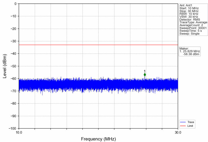
n2_15kHz_SISO_NTNV_10MHz_DFT-s-OFDM_QPSK_1905MHz_Edge_1RB_Right
