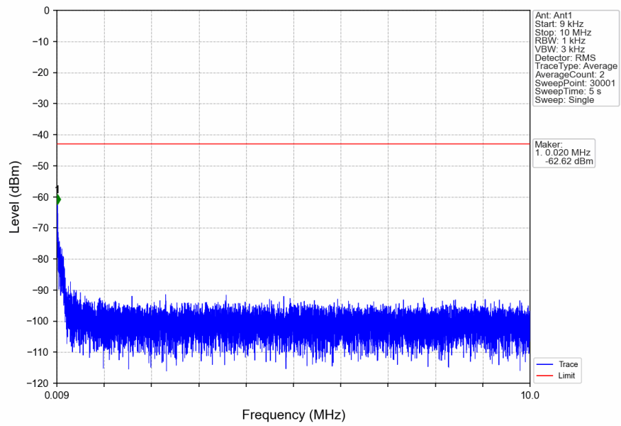
n2_15kHz_SISO_NTNV_10MHz_DFT-s-OFDM_QPSK_1905MHz_Inner_1RB_Right
