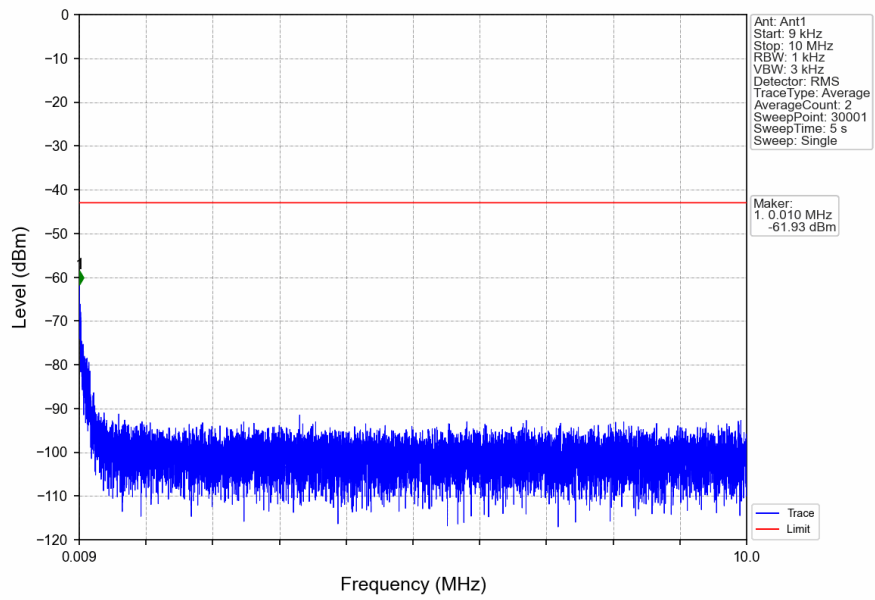
n2_15kHz_SISO_NTNV_10MHz_CP-OFDM_QPSK_1880MHz_Edge_1RB_Left
