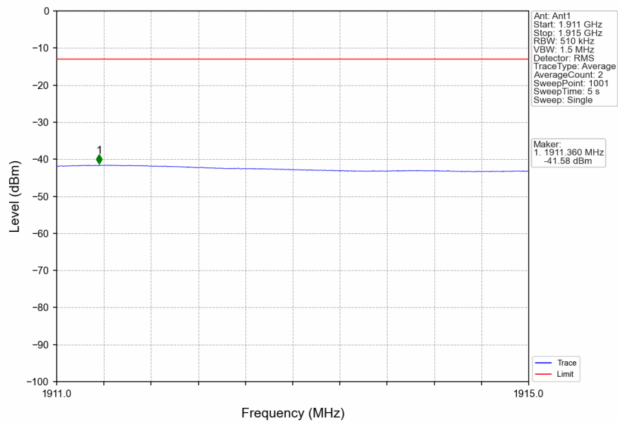
n2_15kHz_SISO_NTNV_10MHz_DFT-s-OFDM_QPSK_1905MHz_Outer_Full
