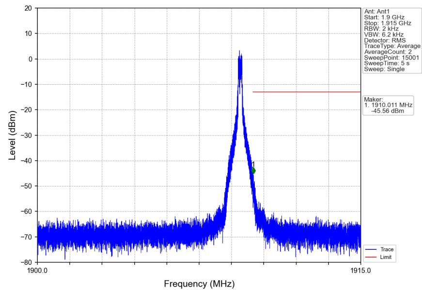
n2_15kHz_SISO_NTNV_10MHz_DFT-s-OFDM_QPSK_1905MHz_Inner_1RB_Right
