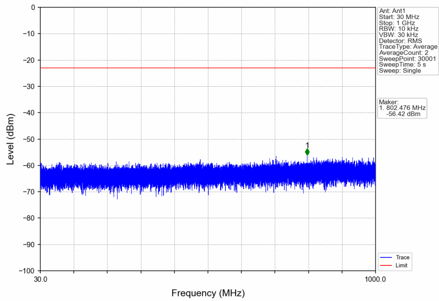
n2_15kHz_SISO_NTNV_10MHz_DFT-s-OFDM_QPSK_1905MHz_Edge_1RB_Right
