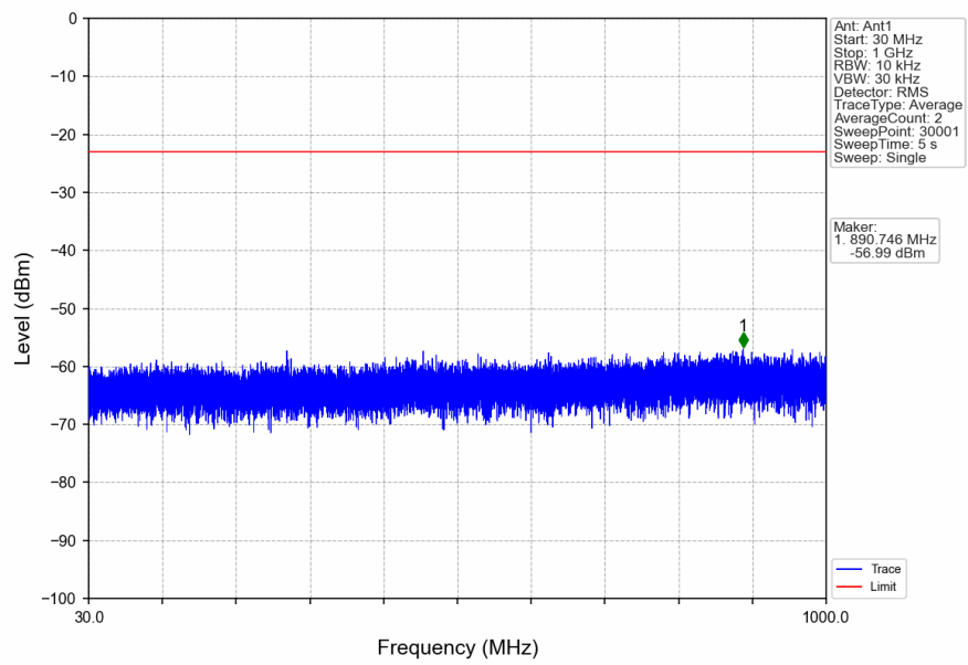
n2_15kHz_SISO_NTNV_10MHz_DFT-s-OFDM_QPSK_1880MHz_Edge_1RB_Left
