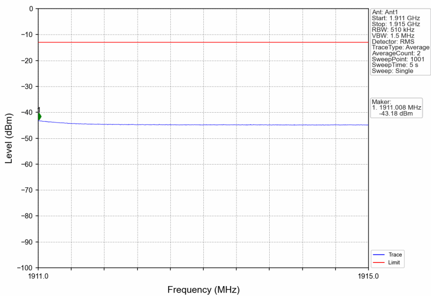
n2_15kHz_SISO_NTNV_5MHz_CP-OFDM_QPSK_1907.5MHz_Inner_1RB_Right
