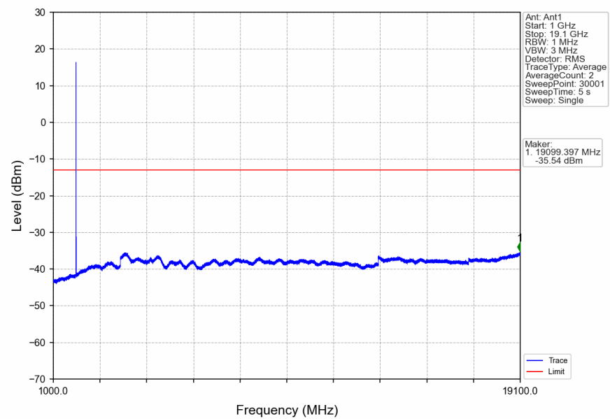
n2_15kHz_SISO_NTNV_10MHz_DFT-s-OFDM_QPSK_1880MHz_Edge_1RB_Left
