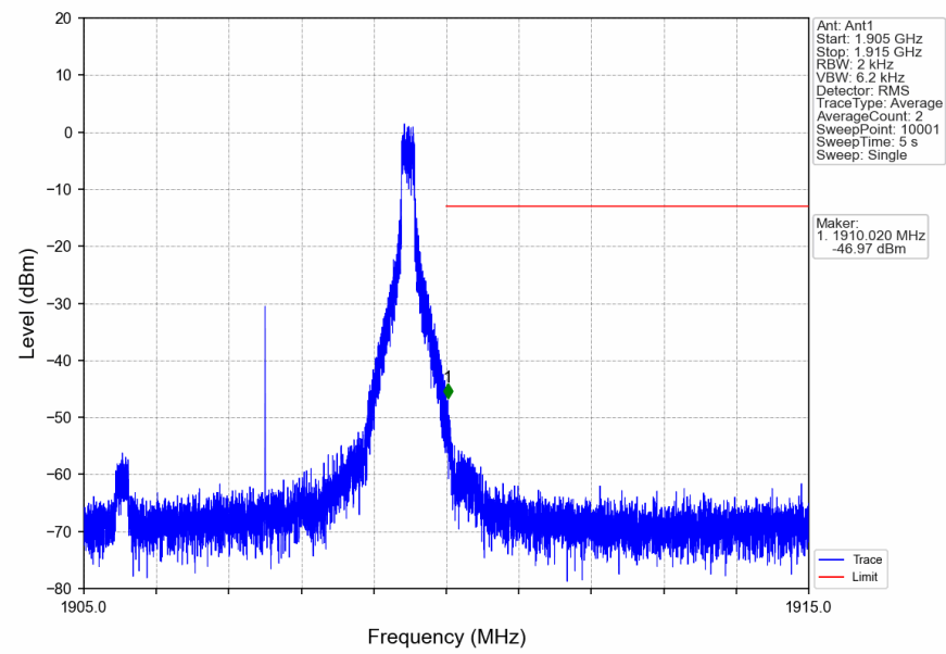
n2_15kHz_SISO_NTNV_5MHz_CP-OFDM_QPSK_1907.5MHz_Inner_1RB_Right
