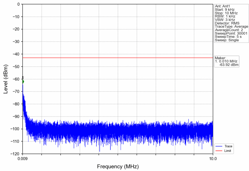
n2_15kHz_SISO_NTNV_10MHz_DFT-s-OFDM_QPSK_1905MHz_Edge_1RB_Right
