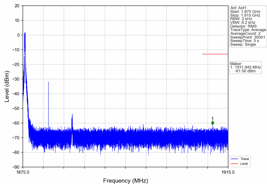
n2_15kHz_SISO_NTNV_10MHz_DFT-s-OFDM_QPSK_1880MHz_Edge_1RB_Left
