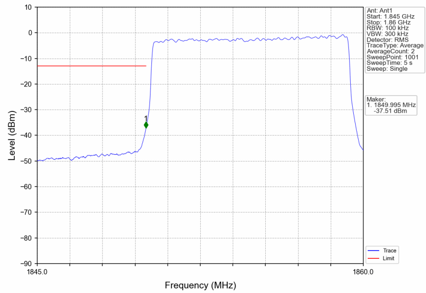
n2_15kHz_SISO_NTNV_10MHz_DFT-s-OFDM_QPSK_1855MHz_Outer_Full
