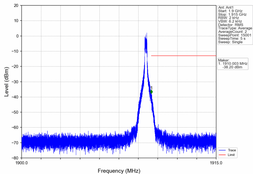
n2_15kHz_SISO_NTNV_10MHz_CP-OFDM QPSK_1905MHz_Edge_1RB_Right
