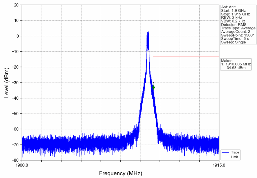
n2_15kHz_SISO_NTNV_10MHz_DFT-s-OFDM_QPSK_1905MHz_Edge_1RB_Right
