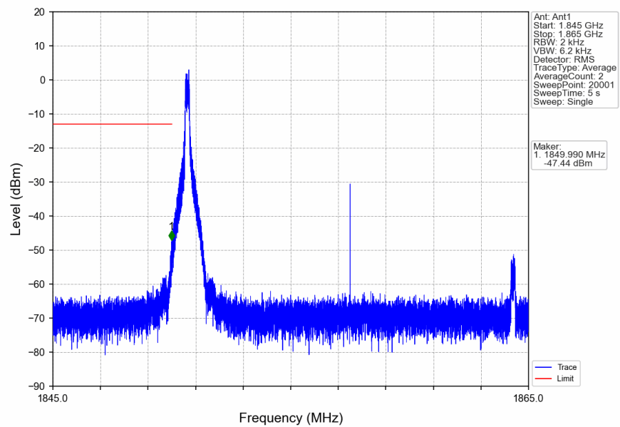
n2_15kHz_SISO_NTNV_15MHz_DFT-s-OFDM_QPSK_1857.5MHz_Inner_1RB_Left
