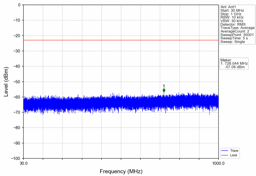
n2_15kHz_SISO_NTNV_15MHz_DFT-s-OFDM_QPSK_1857.5MHz_Edge_1RB_Left
