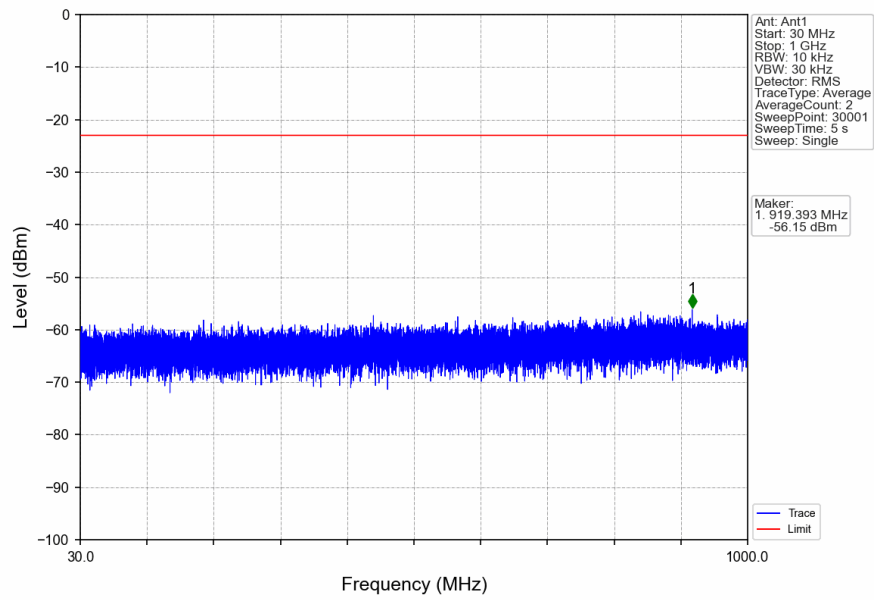
n2_15kHz_SISO_NTNV_15MHz_DFT-s-OFDM_QPSK_1902.5MHz_Inner_1RB_Right
