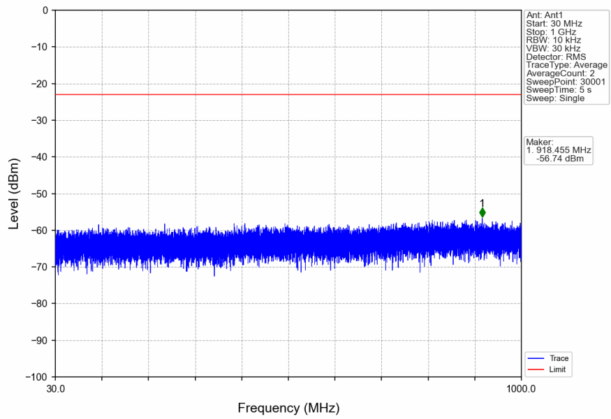
n2_15kHz_SISO_NTNV_10MHz_CP-OFDM QPSK_1905MHz_Edge_1RB_Right
