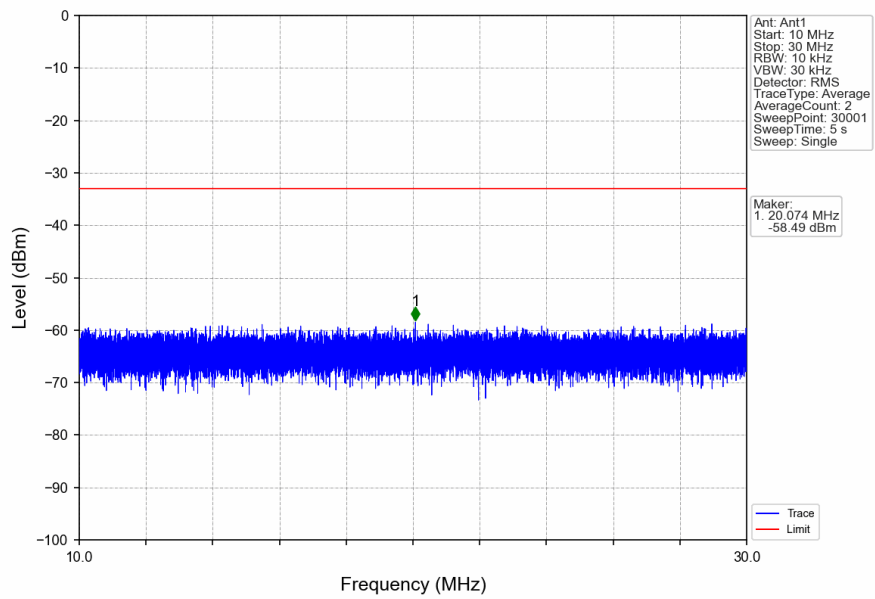
n2_15kHz_SISO_NTNV_15MHz_CP-OFDM_QPSK_1857.5MHz_Edge_1RB_Left
