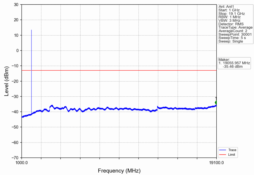
n2_15kHz_SISO_NTNV_10MHz_CP-OFDM QPSK_1905MHz_Edge_1RB_Right
