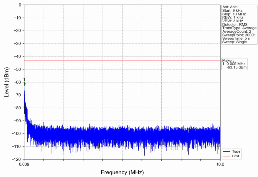
n2_15kHz_SISO_NTNV_15MHz_DFT-s-OFDM_QPSK_1880MHz_Edge_1RB_Left
