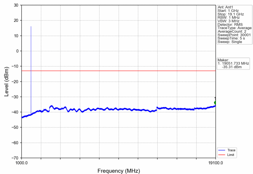
n2_15kHz_SISO_NTNV_15MHz_DFT-s-OFDM_QPSK_1880MHz_Edge_1RB_Left
