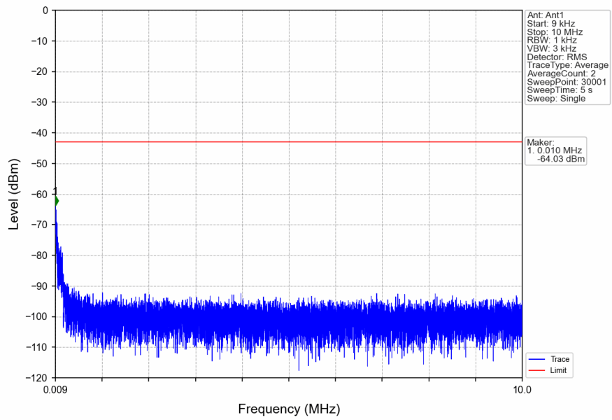
n2_15kHz_SISO_NTNV_15MHz_DFT-s-OFDM_QPSK_1857.5MHz_Inner_1RB_Left
