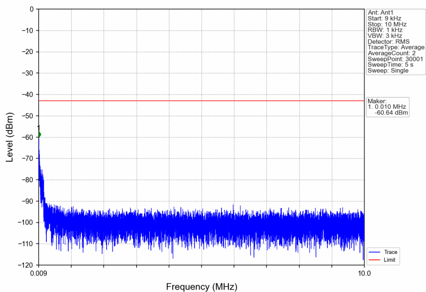
n2_15kHz_SISO_NTNV_15MHz_DFT-s-OFDM_QPSK_1902.5MHz_Edge_1RB_Right
