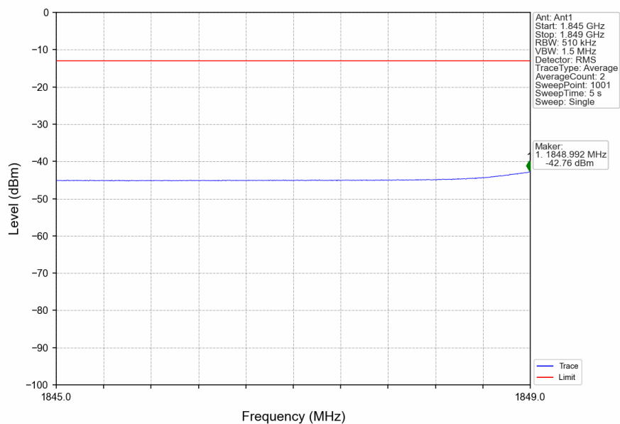
n2_15kHz_SISO_NTNV_15MHz_DFT-s-OFDM_QPSK_1857.5MHz_Edge_1RB_Left
