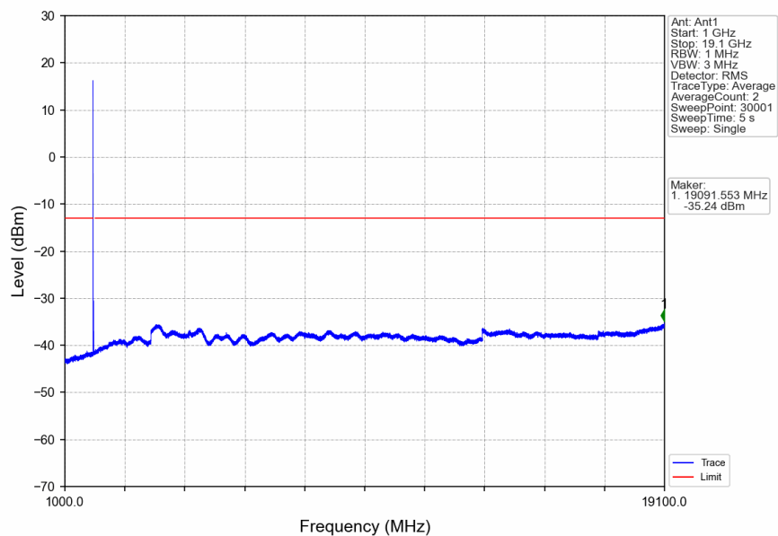
n2_15kHz_SISO_NTNV_15MHz_DFT-s-OFDM_QPSK_1857.5MHz_Inner_1RB_Left
