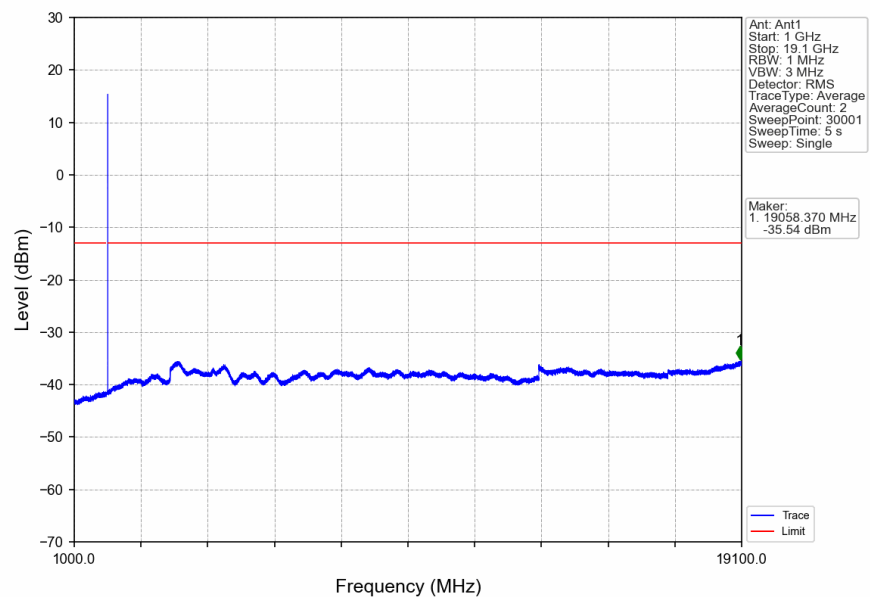
n2_15kHz_SISO_NTNV_15MHz_DFT-s-OFDM_QPSK_1902.5MHz_Edge_1RB_Right
