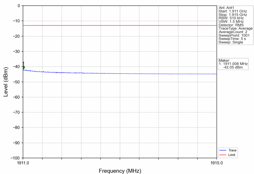
n2_15kHz_SISO_NTNV_15MHz_DFT-s-OFDM_QPSK_1902.5MHz_Edge_1RB_Right
