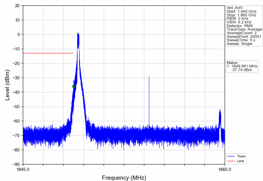
n2_15kHz_SISO_NTNV_15MHz_DFT-s-OFDM_QPSK_1857.5MHz_Edge_1RB_Left
