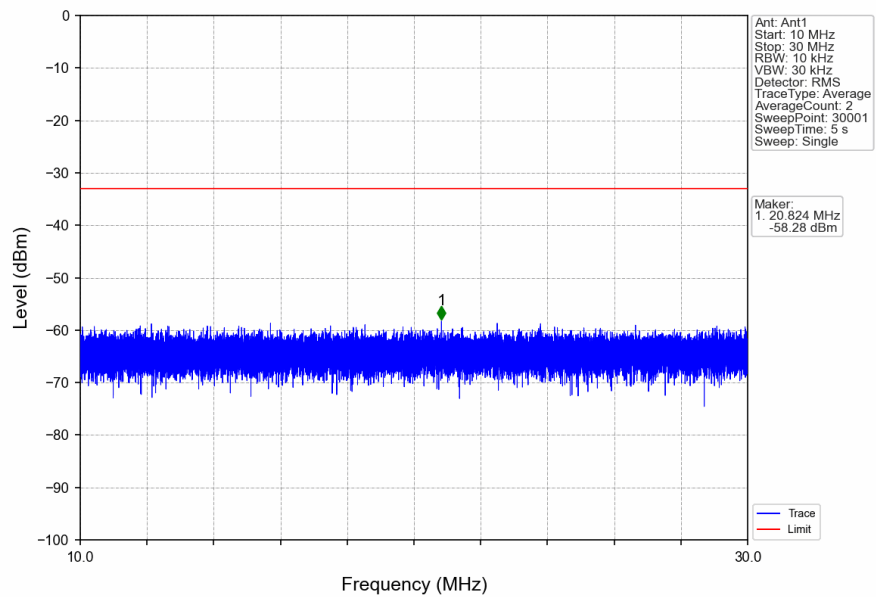
n2_15kHz_SISO_NTNV_15MHz_DFT-s-OFDM_QPSK_1857.5MHz_Edge_1RB_Left
