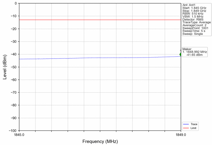
n2_15kHz_SISO_NTNV_15MHz_DFT-s-OFDM_QPSK_1857.5MHz_Outer_Full
