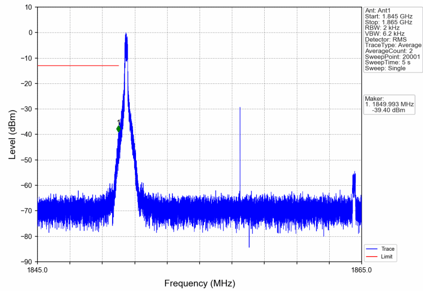
n2_15kHz_SISO_NTNV_15MHz_CP-OFDM_QPSK_1857.5MHz_Edge_1RB_Left
