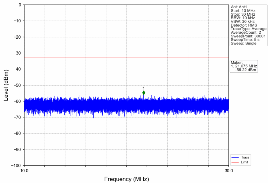
n2_15kHz_SISO_NTNV_15MHz_DFT-s-OFDM_PI/2_BPSK_1902.5MHz_Edge_1RB_Right
