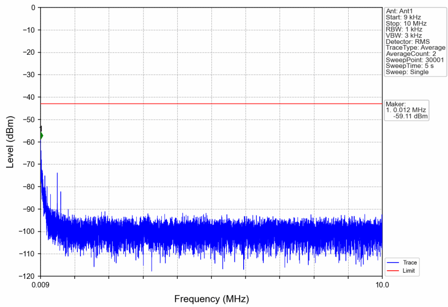
n2_15kHz_SISO_NTNV_15MHz_DFT-s-OFDM_PI/2_BPSK_1902.5MHz_Edge_1RB_Right
