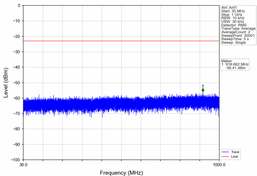
n2_15kHz_SISO_NTNV_15MHz_DFT-s-OFDM_QPSK_1880MHz_Edge_1RB_Left
