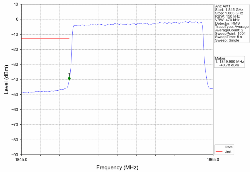
n2_15kHz_SISO_NTNV_15MHz_DFT-s-OFDM_QPSK_1857.5MHz_Outer_Full
