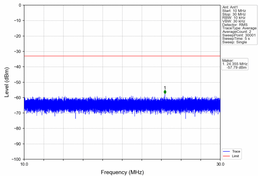
n2_15kHz_SISO_NTNV_15MHz_DFT-s-OFDM_QPSK_1880MHz_Edge_1RB_Left
