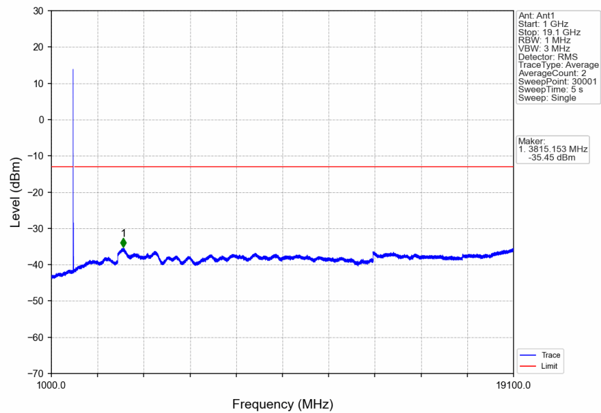
n2_15kHz_SISO_NTNV_15MHz_CP-OFDM_QPSK_1857.5MHz_Edge_1RB_Left
