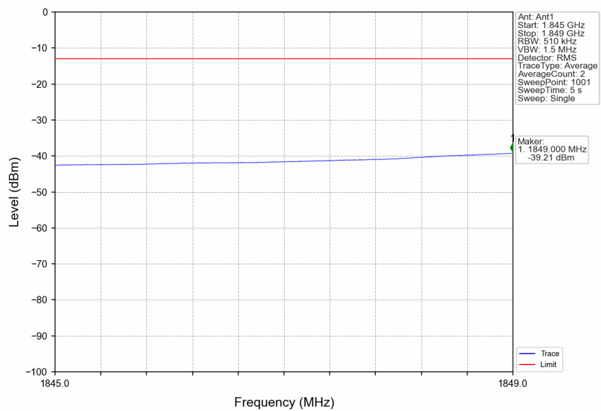
n2_15kHz_SISO_NTNV_15MHz_CP-OFDM_QPSK_1857.5MHz_Outer_Full
