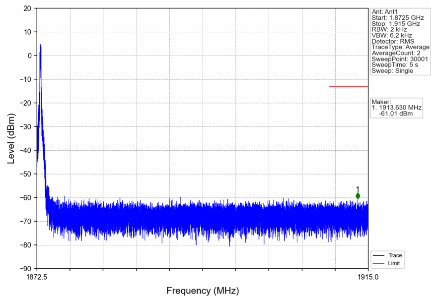
n2_15kHz_SISO_NTNV_15MHz_DFT-s-OFDM_PI/2_BPSK_1880MHz_Edge_1RB_Left
