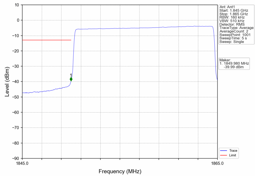
n2_15kHz_SISO_NTNV_15MHz_CP-OFDM_QPSK_1857.5MHz_Outer_Full
