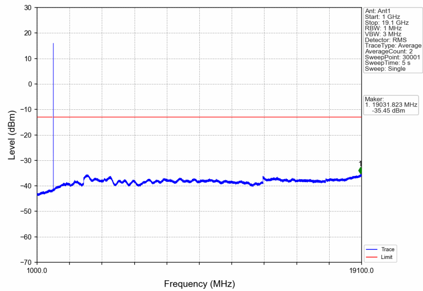
n2_15kHz_SISO_NTNV_20MHz_DFT-s-OFDM_QPSK_1900MHz_Edge_1RB_Right
