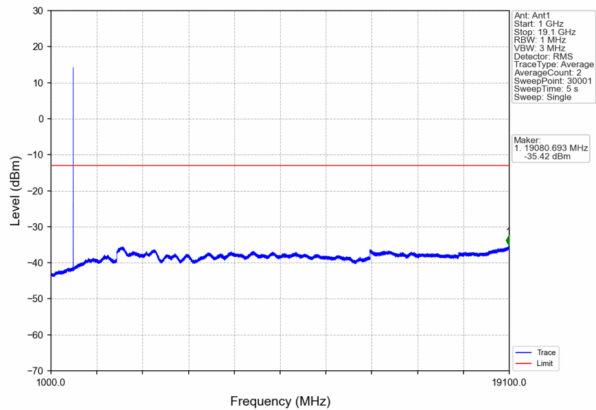
n2_15kHz_SISO_NTNV_15MHz_CP-OFDM_QPSK_1880MHz_Edge_1RB_Left
