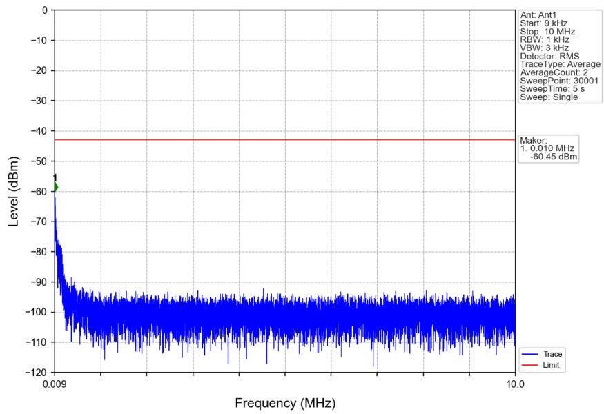
n2_15kHz_SISO_NTNV_15MHz_CP-OFDM QPSK_1902.5MHz_Inner_1RB_Right
