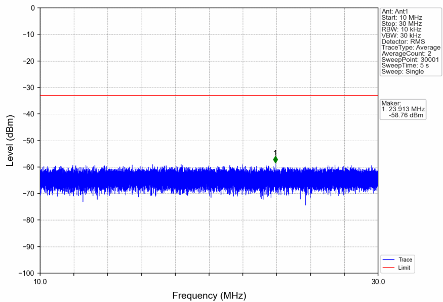
n2_15kHz_SISO_NTNV_15MHz_CP-OFDM QPSK_1902.5MHz_Inner_1RB_Right
