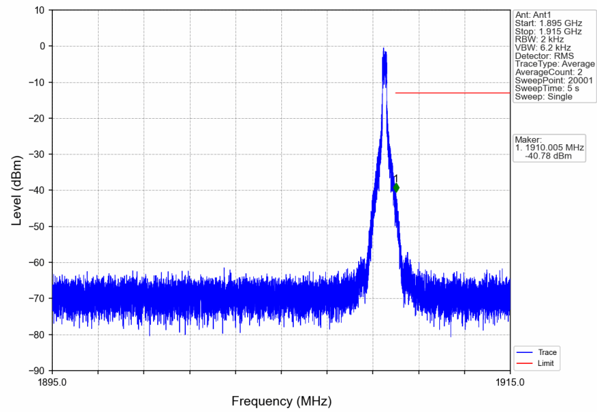
n2_15kHz_SISO_NTNV_15MHz_CP-OFDM QPSK_1902.5MHz_Edge_1RB_Right
