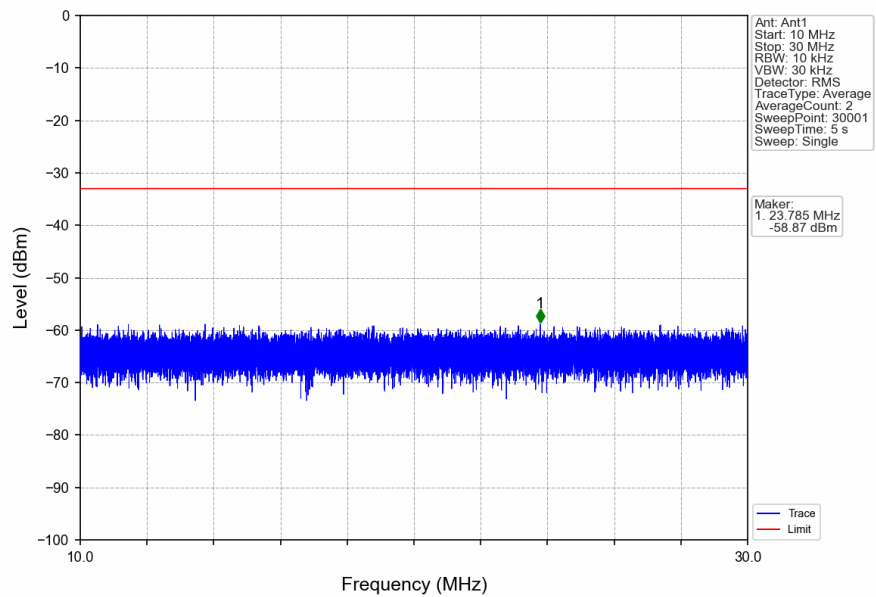
n2_15kHz_SISO_NTNV_20MHz_DFT-s-OFDM_QPSK_1900MHz_Edge_1RB_Right
