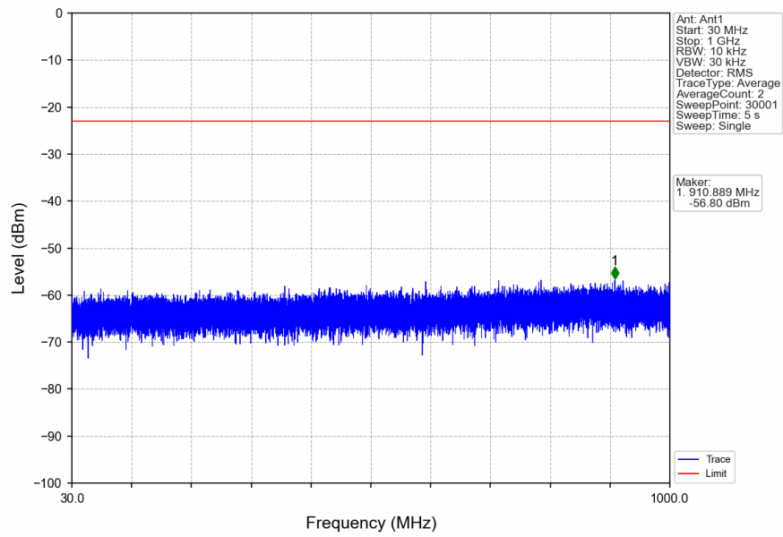
n2_15kHz_SISO_NTNV_20MHz_DFT-s-OFDM_QPSK_1900MHz_Edge_1RB_Right
