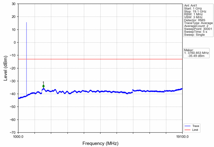
n2_15kHz_SISO_NTNV_15MHz_CP-OFDM QPSK_1902.5MHz_Inner_1RB_Right
