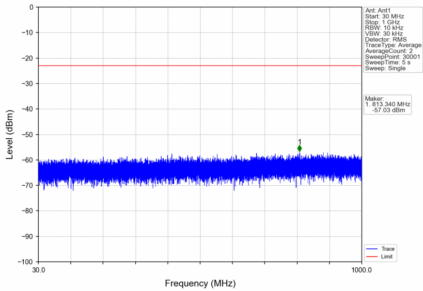
n2_15kHz_SISO_NTNV_15MHz_CP-OFDM_QPSK_1880MHz_Edge_1RB_Left
