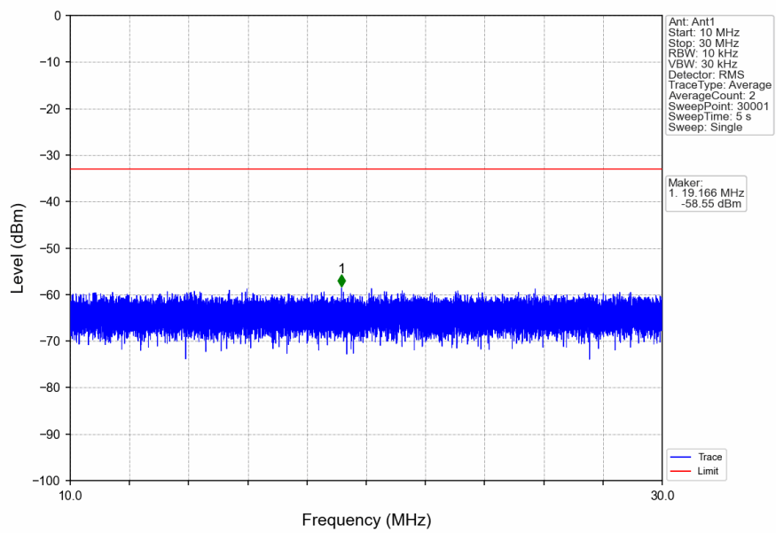
n2_15kHz_SISO_NTNV_15MHz_CP-OFDM QPSK_1902.5MHz_Edge_1RB_Right
