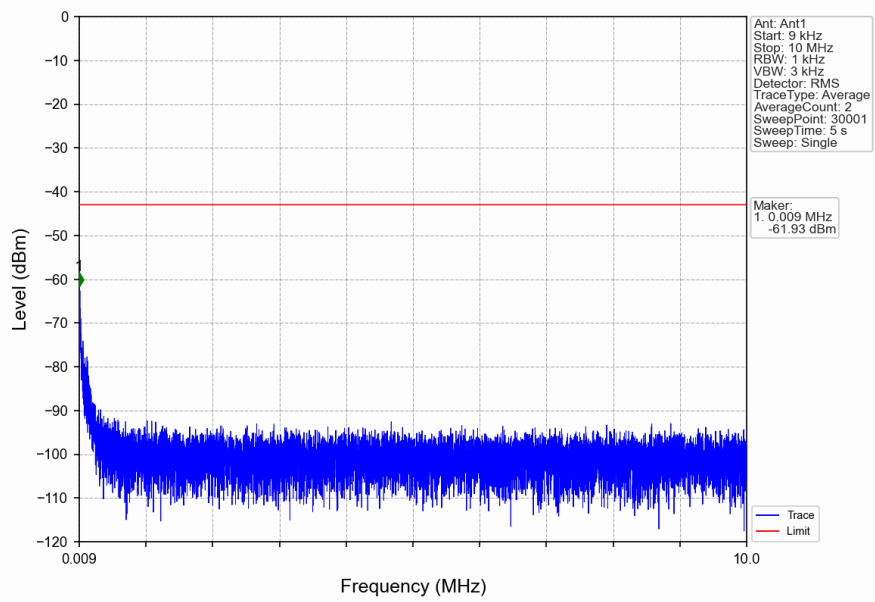
n2_15kHz_SISO_NTNV_15MHz_CP-OFDM QPSK_1902.5MHz_Edge_1RB_Right
