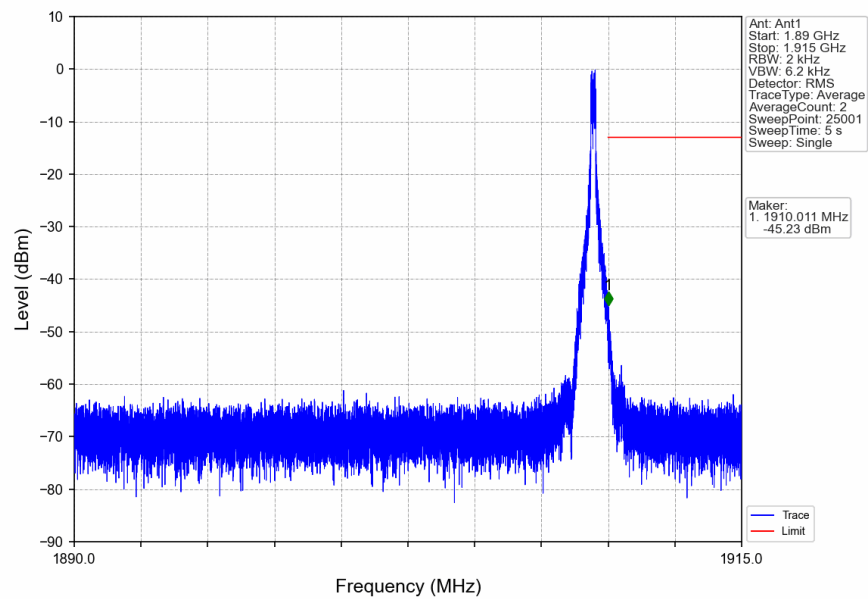
n2_15kHz_SISO_NTNV_20MHz_CP-OFDM QPSK_1900MHz_Edge_1RB_Right
