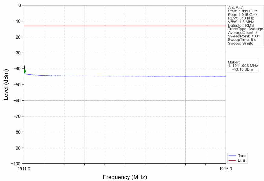
n2_15kHz_SISO_NTNV_20MHz_CP-OFDM QPSK_1900MHz_Edge_1RB_Right
