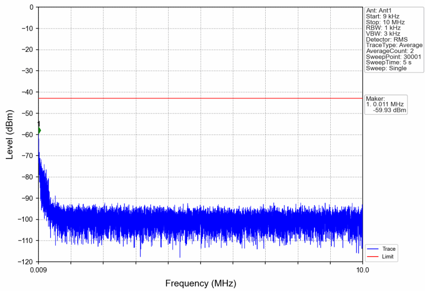
n41_30kHz_SISO_NTNV_30MHz_CP-OFDM_QPSK_2511MHz_Edge_1RB_Left
