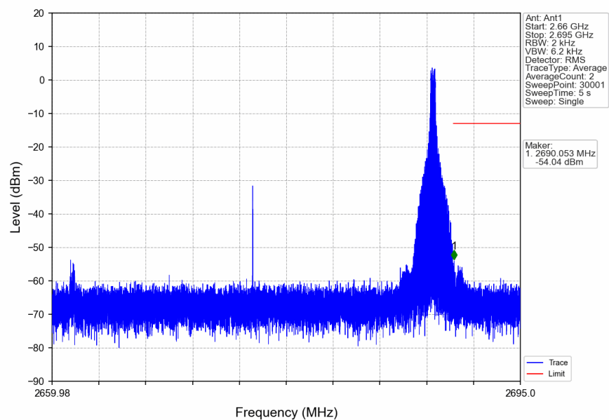
n41_30kHz_SISO_NTNV_30MHz_DFT-s-OFDM_QPSK_2674.98MHz_Inner_1RB_Right
