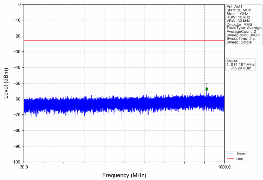
n41_30kHz_SISO_NTNV_30MHz_DFT-s-OFDM_QPSK_2511MHz_Edge_1RB_Left
