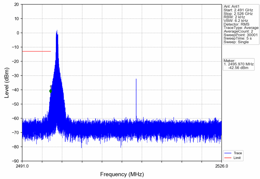
n41_30kHz_SISO_NTNV_30MHz_CP-OFDM_QPSK_2511MHz_Edge_1RB_Left
