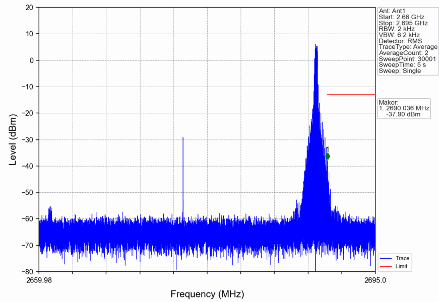
n41_30kHz_SISO_NTNV_30MHz_DFT-s-OFDM_PI/2_BPSK_2674.98MHz_Edge_1RB_Right
