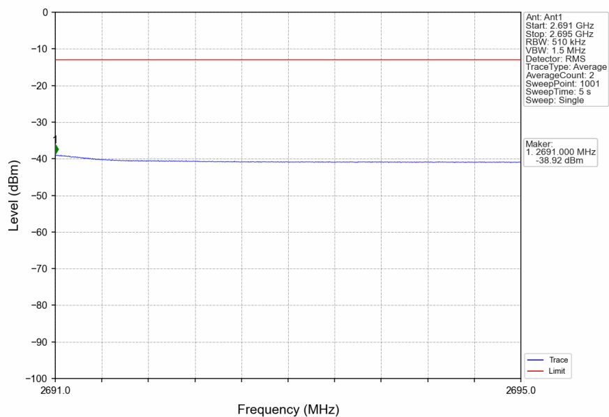
n41_30kHz_SISO_NTNV_30MHz_DFT-s-OFDM_QPSK_2674.98MHz_Edge_1RB_Right
