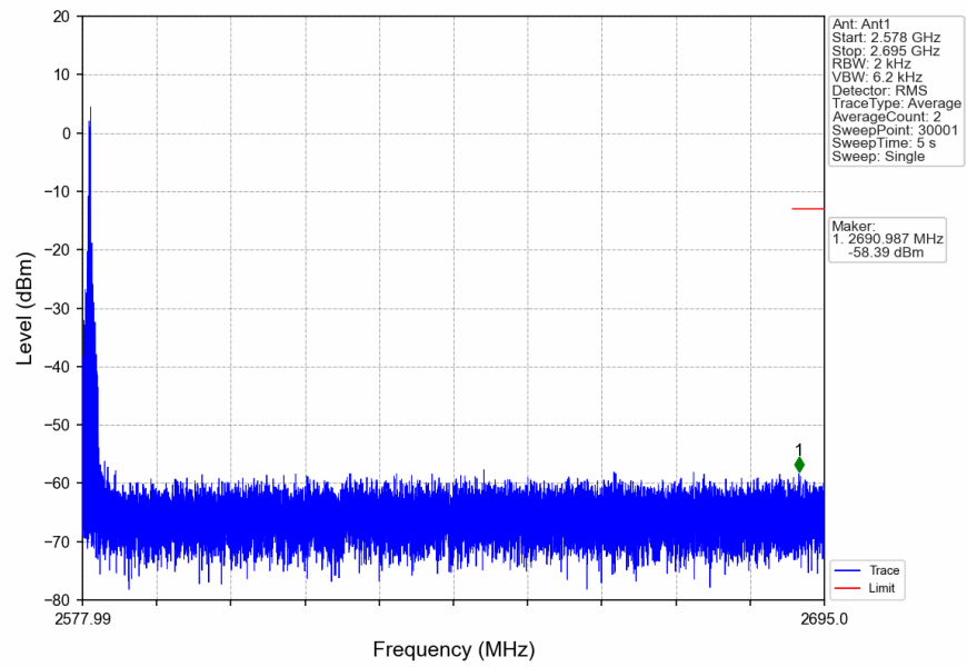
n41_30kHz_SISO_NTNV_30MHz_DFT-s-OFDM PI/2 BPSK_2592.99MHz_Edge_1RB_Left
