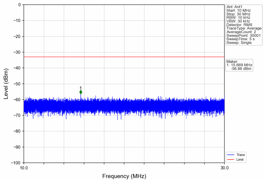
n41_30kHz_SISO_NTNV_30MHz_DFT-s-OFDM_QPSK_2511MHz_Edge_1RB_Left
