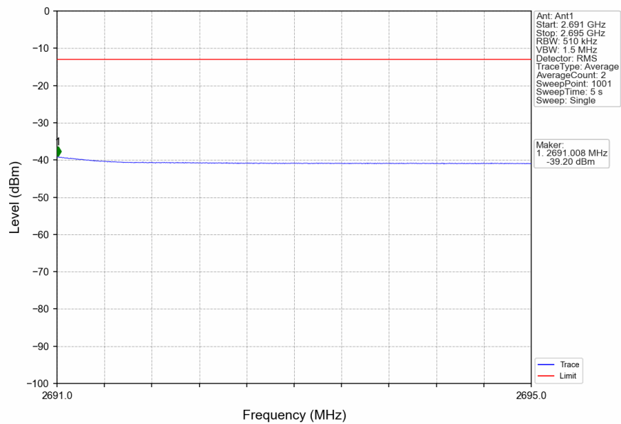
n41_30kHz_SISO_NTNV_30MHz_DFT-s-OFDM_PI/2_BPSK_2674.98MHz_Edge_1RB_Right
