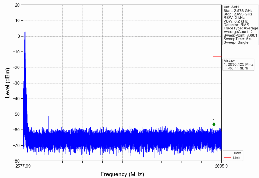
n41_30kHz_SISO_NTNV_30MHz_DFT-s-OFDM_QPSK_2592.99MHz_Edge_1RB_Left
