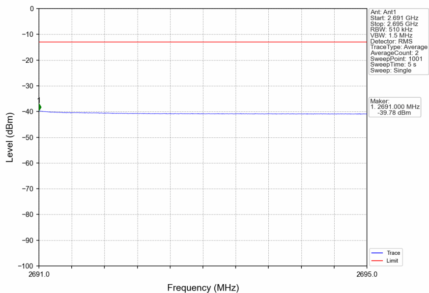
n41_30kHz_SISO_NTNV_30MHz_DFT-s-OFDM_QPSK_2674.98MHz_Inner_1RB_Right
