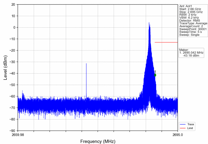
n41_30kHz_SISO_NTNV_30MHz_DFT-s-OFDM_QPSK_2674.98MHz_Edge_1RB_Right
