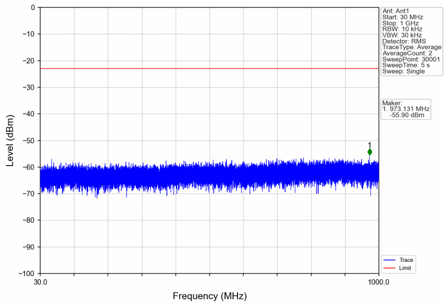
n41_30kHz_SISO_NTNV_30MHz_DFT-s-OFDM_QPSK_2592.99MHz_Edge_1RB_Left
