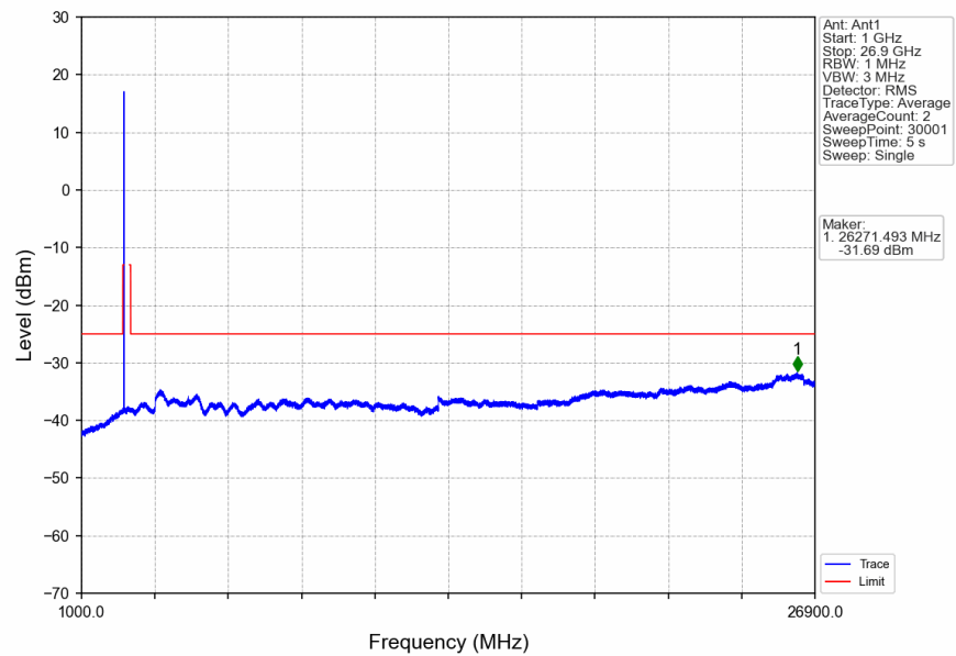
n41_30kHz_SISO_NTNV_40MHz_CP-OFDM_QPSK_2516.01MHz_Edge_1RB_Left
