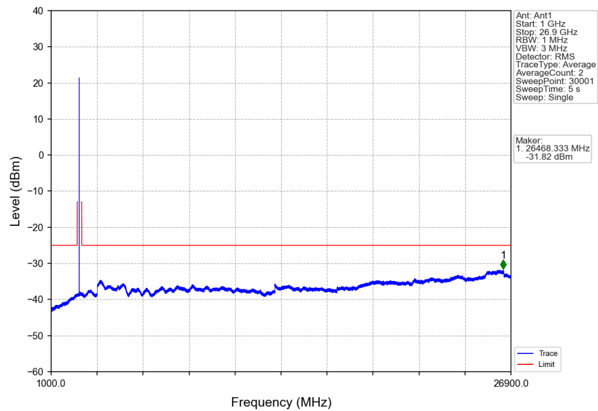
n41_30kHz_SISO_NTNV_30MHz_CP-OFDM_QPSK_2592.99MHz_Edge_1RB_Left
