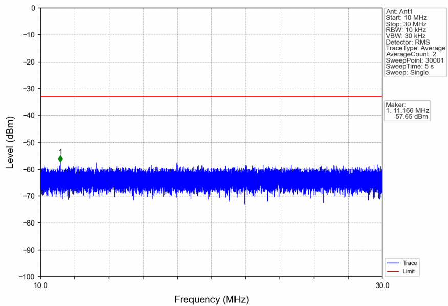
n41_30kHz_SISO_NTNV_30MHz_CP-OFDM_QPSK_2592.99MHz_Edge_1RB_Left
