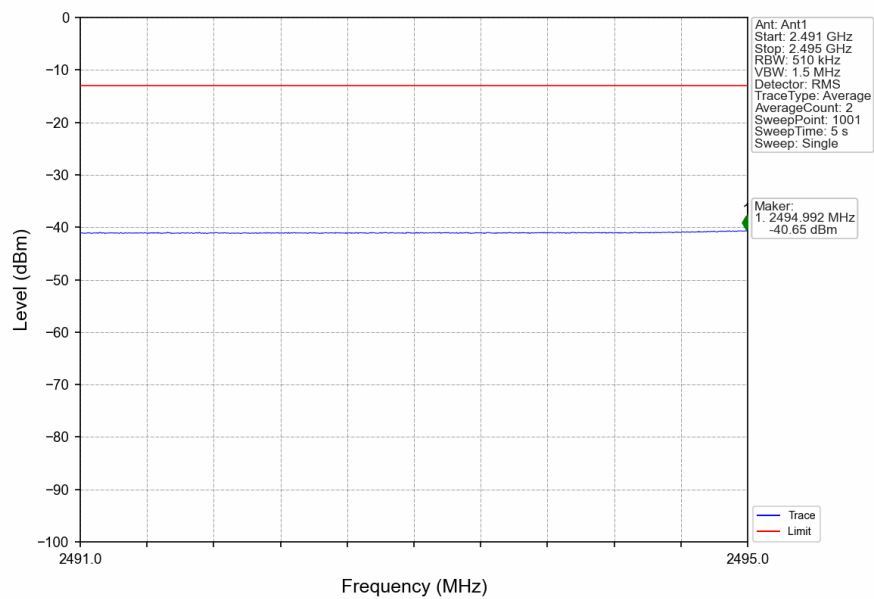
n41_30kHz_SISO_NTNV_40MHz_DFT-s-OFDM_QPSK_2516.01MHz_Edge_1RB_Left
