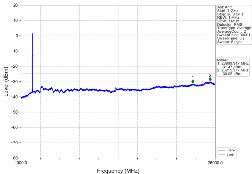
n41_30kHz_SISO_NTNV_40MHz_DFT-s-OFDM_QPSK_2516.01MHz_Outer_Full
