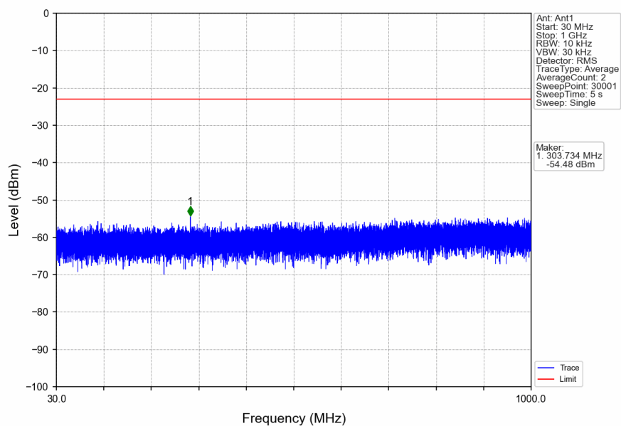
n41_30kHz_SISO_NTNV_40MHz_DFT-s-OFDM_QPSK_2516.01MHz_Outer_Full
