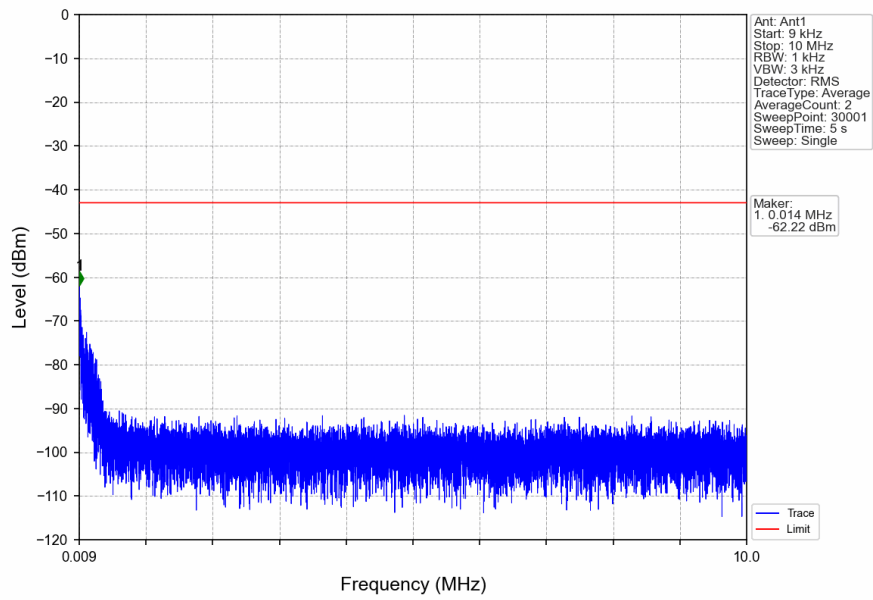
n41_30kHz_SISO_NTNV_40MHz_CP-OFDM_QPSK_2516.01MHz_Edge_1RB_Left
