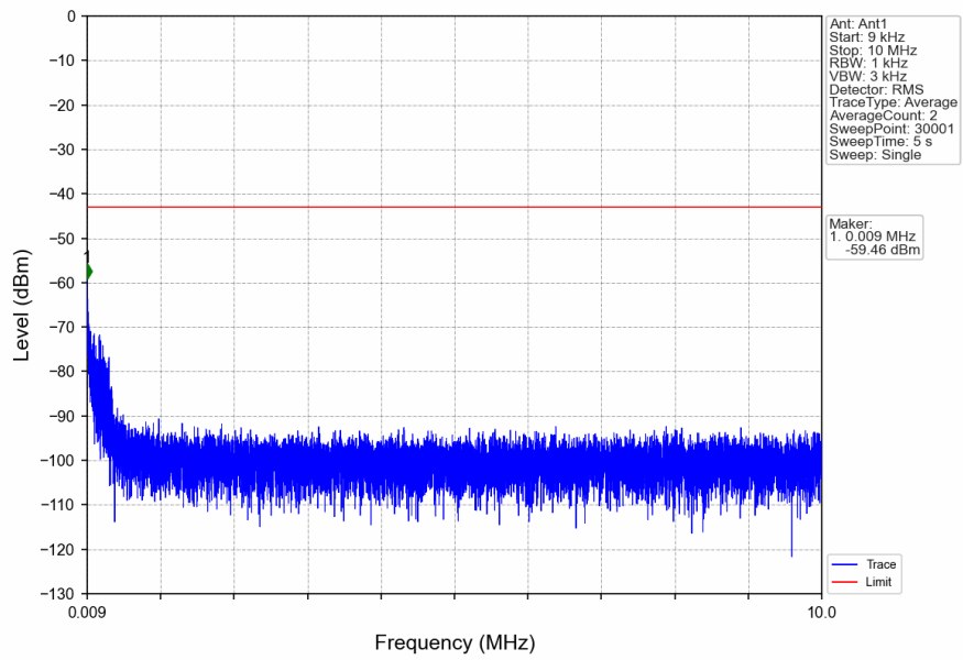
n41_30kHz_SISO_NTNV_30MHz_CP-OFDM_QPSK_2592.99MHz_Edge_1RB_Left
