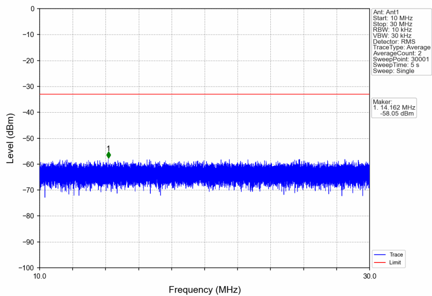
n41_30kHz_SISO_NTNV_40MHz_DFT-s-OFDM_QPSK_2592.99MHz_Edge_1RB_Left
