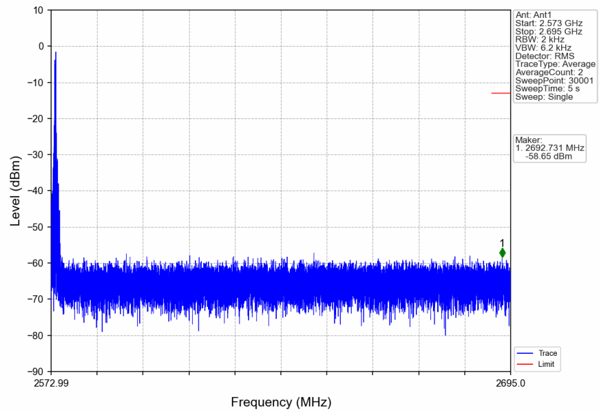
n41_30kHz_SISO_NTNV_40MHz_DFT-s-OFDM PI/2 BPSK_2592.99MHz_Edge_1RB_Left
