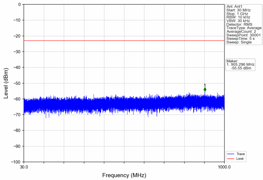
n41_30kHz_SISO_NTNV_40MHz_CP-OFDM_QPSK_2516.01MHz_Edge_1RB_Left
