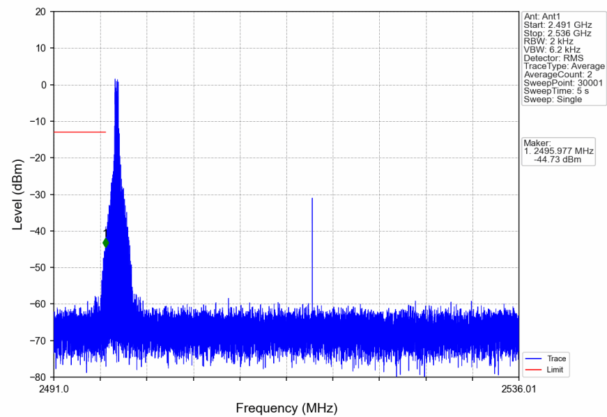
n41_30kHz_SISO_NTNV_40MHz_DFT-s-OFDM_QPSK_2516.01MHz_Edge_1RB_Left
