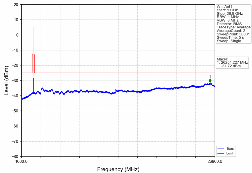
n41_30kHz_SISO_NTNV_50MHz_CP-OFDM_QPSK_2592.99MHz_Edge_1RB_Left
