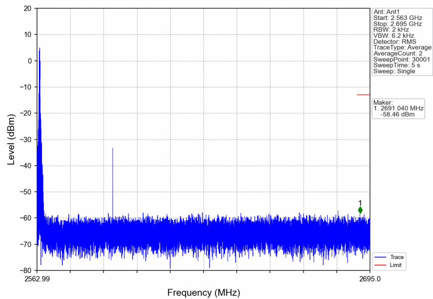
n41_30kHz_SISO_NTNV_60MHz_DFT-s-OFDM_QPSK_2592.99MHz_Edge_1RB_Left
