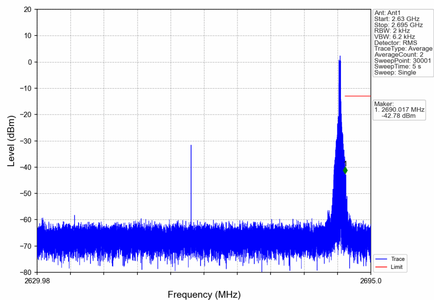
n41_30kHz_SISO_NTNV_60MHz_DFT-s-OFDM_QPSK_2659.98MHz_Edge_1RB_Right
