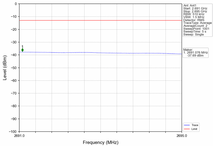
n41_30kHz_SISO_NTNV_60MHz_DFT-s-OFDM_PI/2_BPSK_2659.98MHz_Outer_Full
