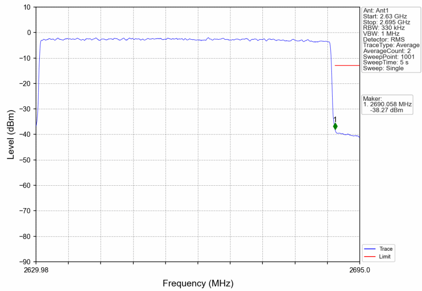
n41_30kHz_SISO_NTNV_60MHz_DFT-s-OFDM_PI/2_BPSK_2659.98MHz_Outer_Full
