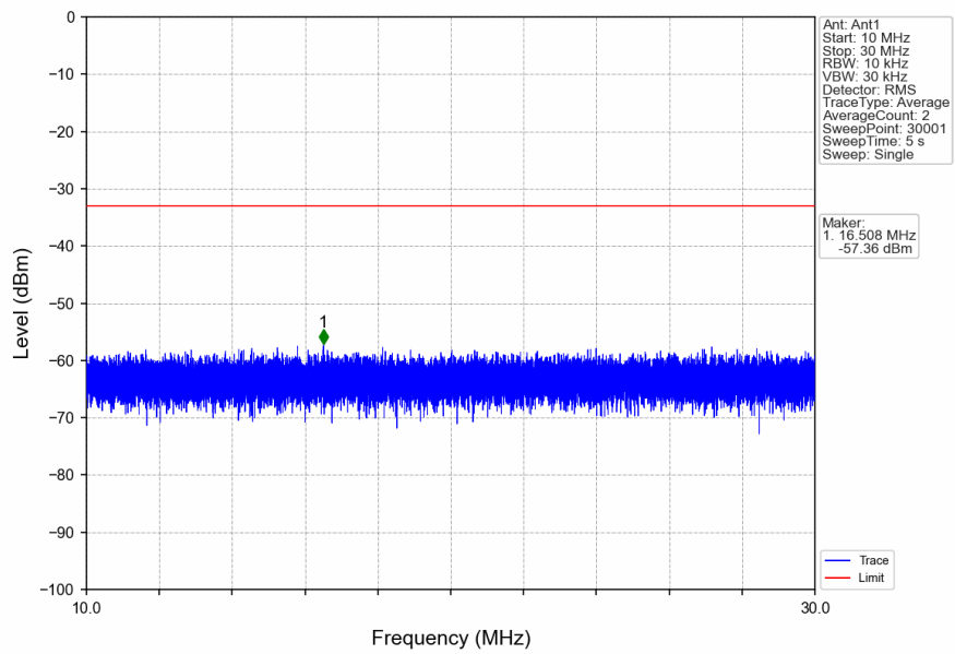
n41_30kHz_SISO_NTNV_60MHz_DFT-s-OFDM_QPSK_2592.99MHz_Edge_1RB_Left
