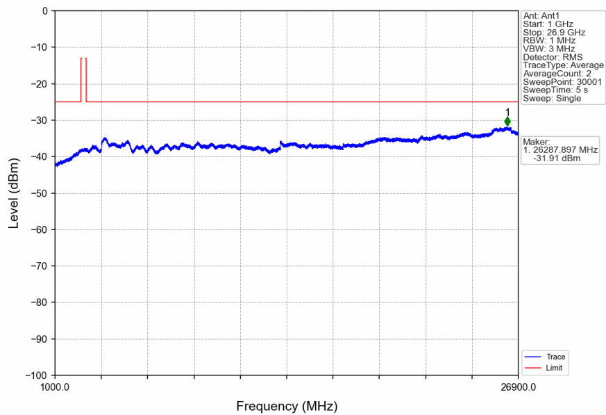
n41_30kHz_SISO_NTNV_50MHz_CP-OFDM_QPSK_2521.02MHz_Edge_1RB_Left
