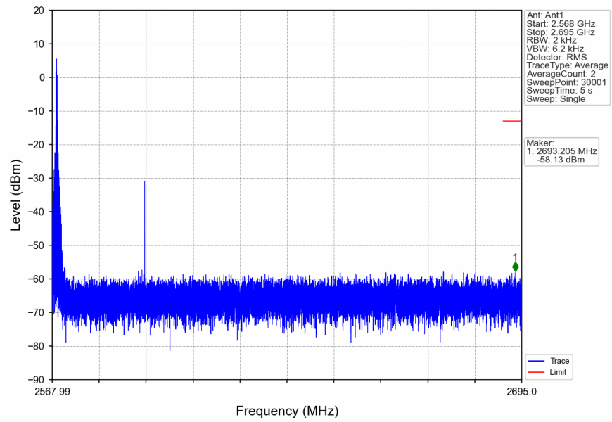
n41_30kHz_SISO_NTNV_50MHz_CP-OFDM_QPSK_2592.99MHz_Edge_1RB_Left
