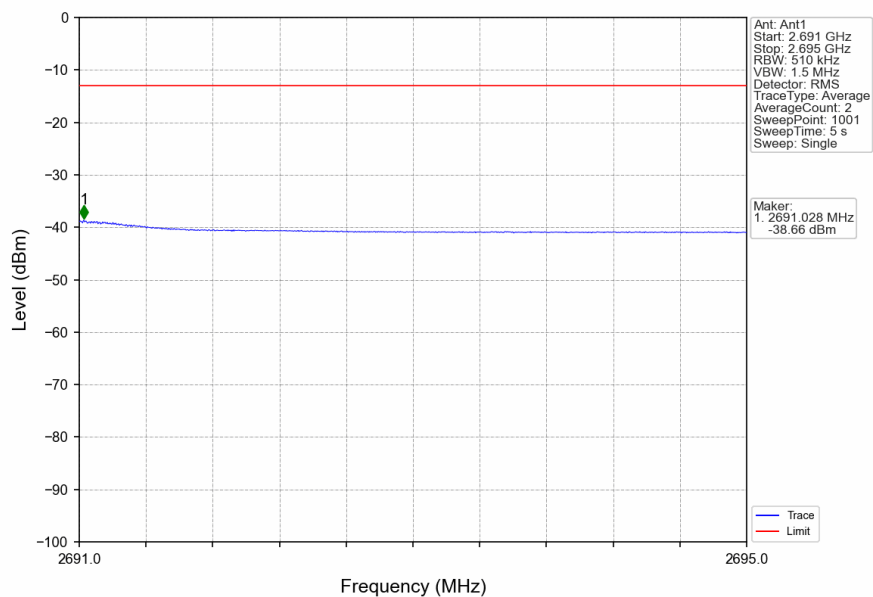
n41_30kHz_SISO_NTNV_60MHz_DFT-s-OFDM_QPSK_2659.98MHz_Edge_1RB_Right
