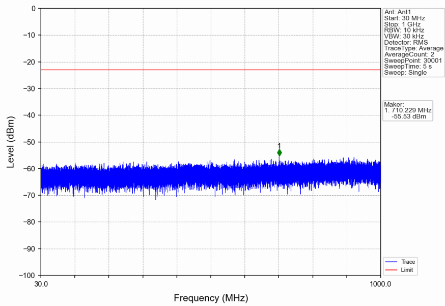
n41_30kHz_SISO_NTNV_60MHz_DFT-s-OFDM_QPSK_2592.99MHz_Edge_1RB_Left
