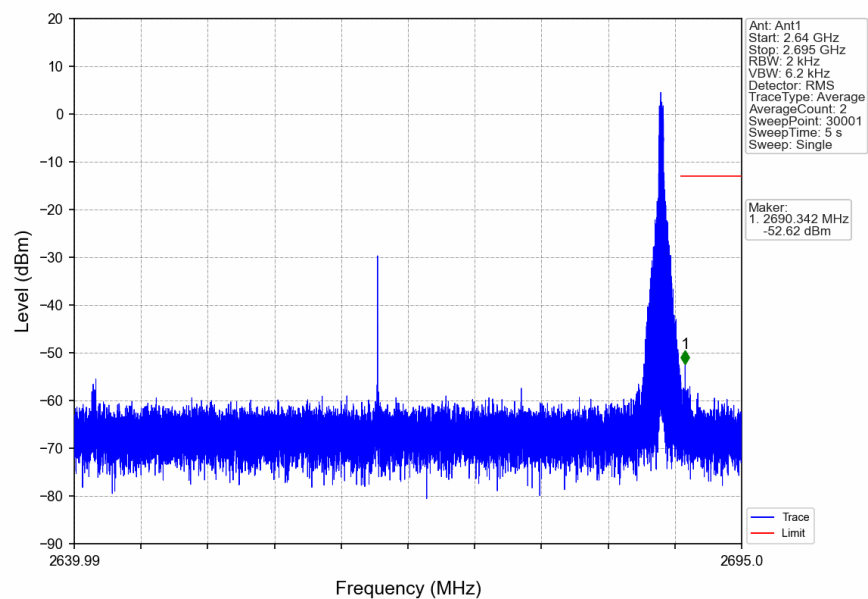
n41_30kHz_SISO_NTNV_50MHz_CP-OFDM QPSK_2664.99MHz_Inner_1RB_Right
