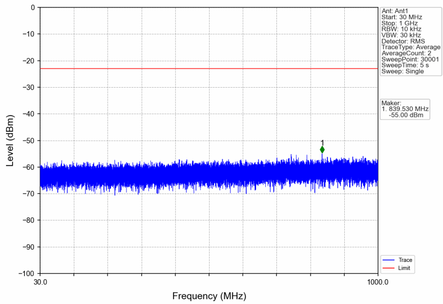
n41_30kHz_SISO_NTNV_50MHz_CP-OFDM_QPSK_2592.99MHz_Edge_1RB_Left
