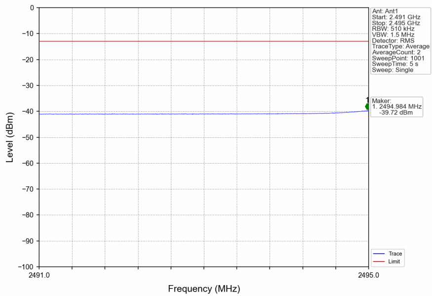
n41_30kHz_SISO_NTNV_50MHz_CP-OFDM_QPSK_2521.02MHz_Edge_1RB_Left
