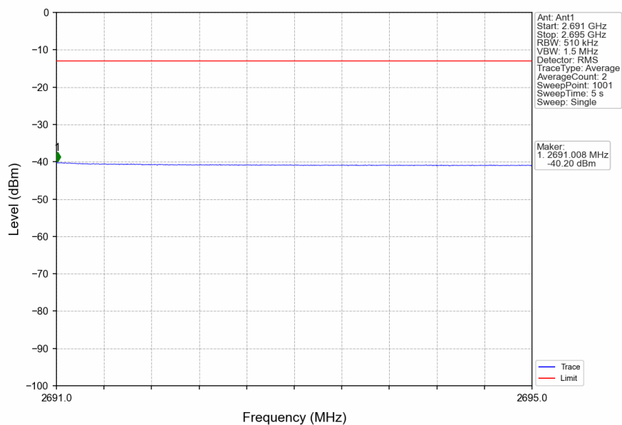
n41_30kHz_SISO_NTNV_50MHz_CP-OFDM QPSK_2664.99MHz_Inner_1RB_Right
