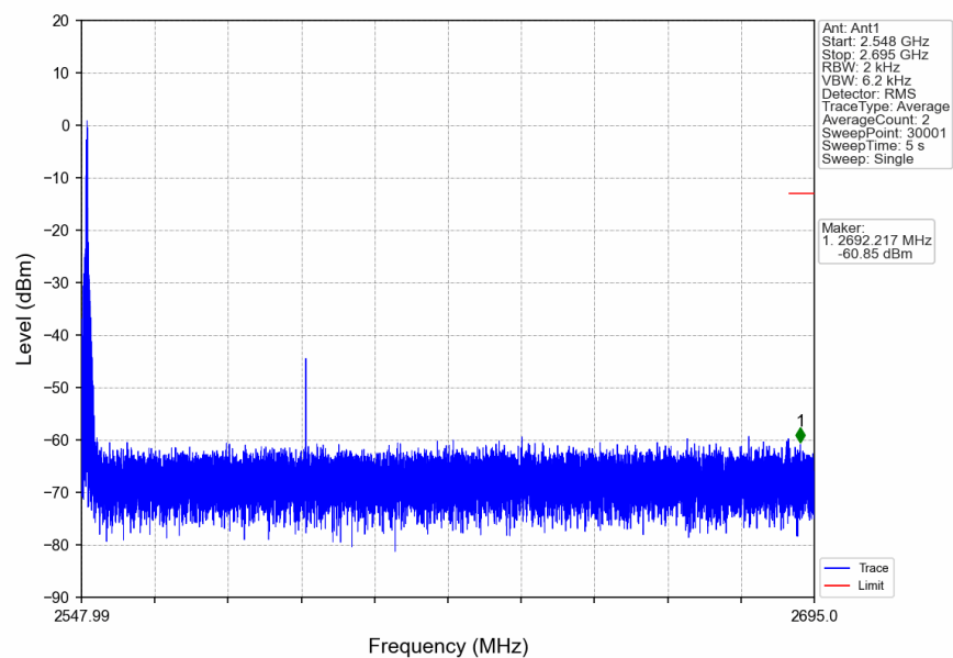
n41_30kHz_SISO_NTNV_90MHz_DFT-s-OFDM PI/2 BPSK_2592.99MHz_Edge_1RB_Left
