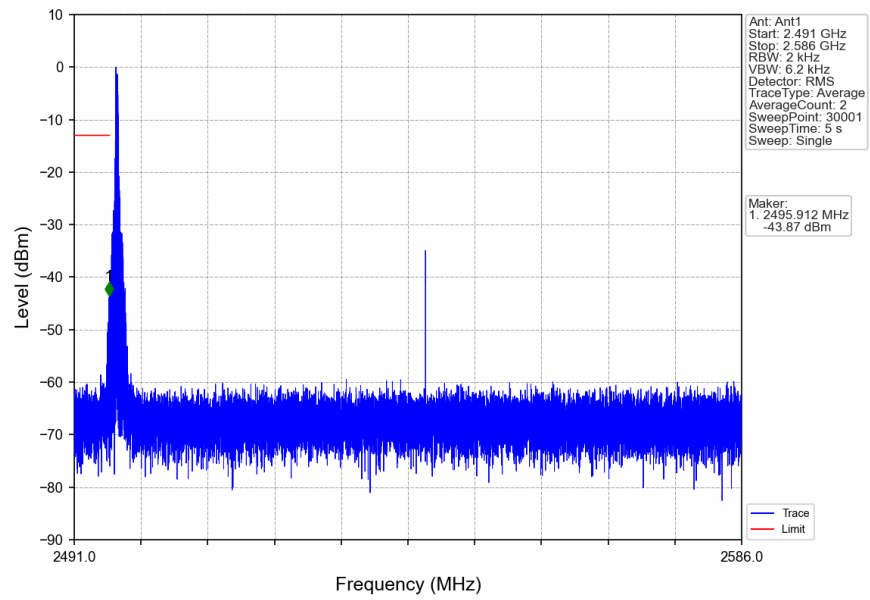
n41_30kHz_SISO_NTNV_90MHz_DFT-s-OFDM_QPSK_2541MHz_Edge_1RB_Left
