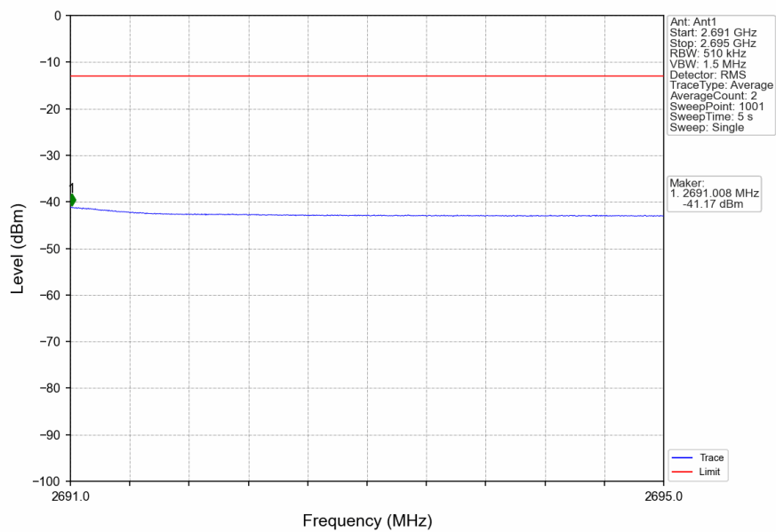
n41_30kHz_SISO_NTNV_80MHz_DFT-s-OFDM_QPSK_2649.99MHz_Edge_1RB_Right
