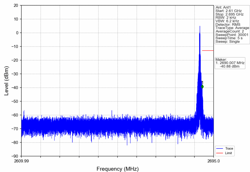
n41_30kHz_SISO_NTNV_80MHz_DFT-s-OFDM_QPSK_2649.99MHz_Edge_1RB_Right
