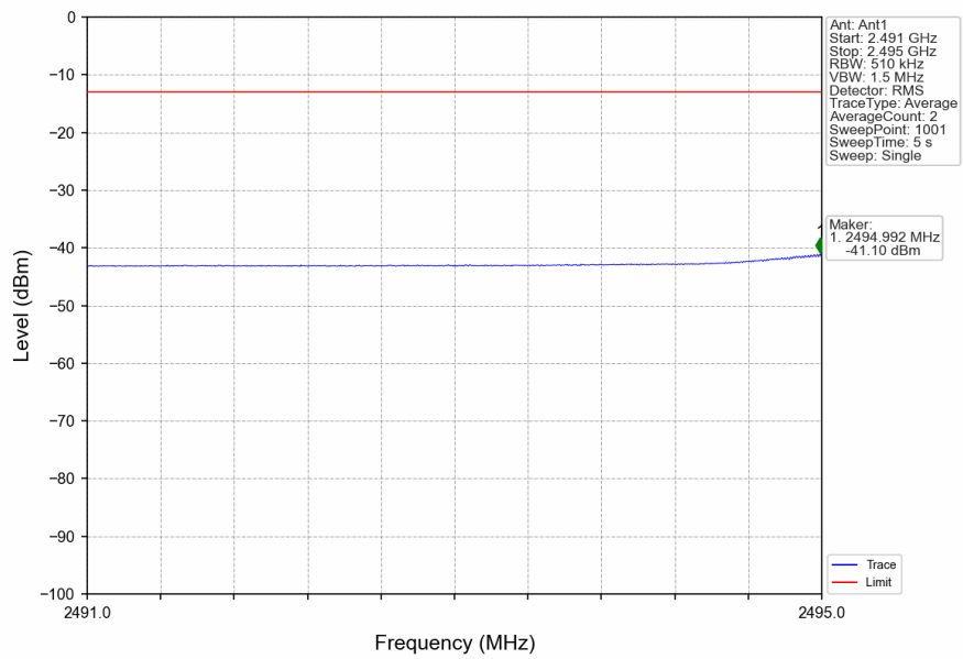
n41_30kHz_SISO_NTNV_80MHz_CP-OFDM_QPSK_2536.02MHz_Edge_1RB_Left
