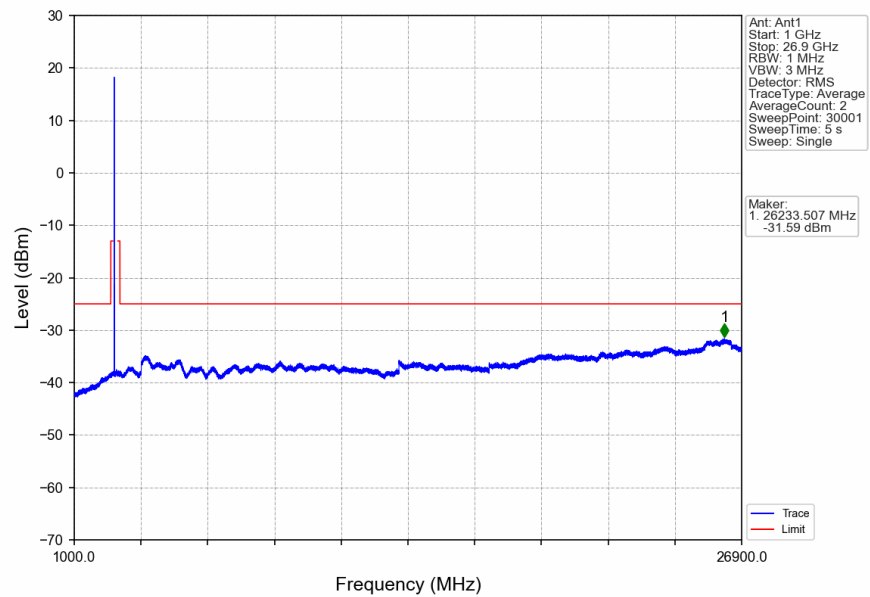
n41_30kHz_SISO_NTNV_80MHz_CP-OFDM_QPSK_2592.99MHz_Edge_1RB_Left
