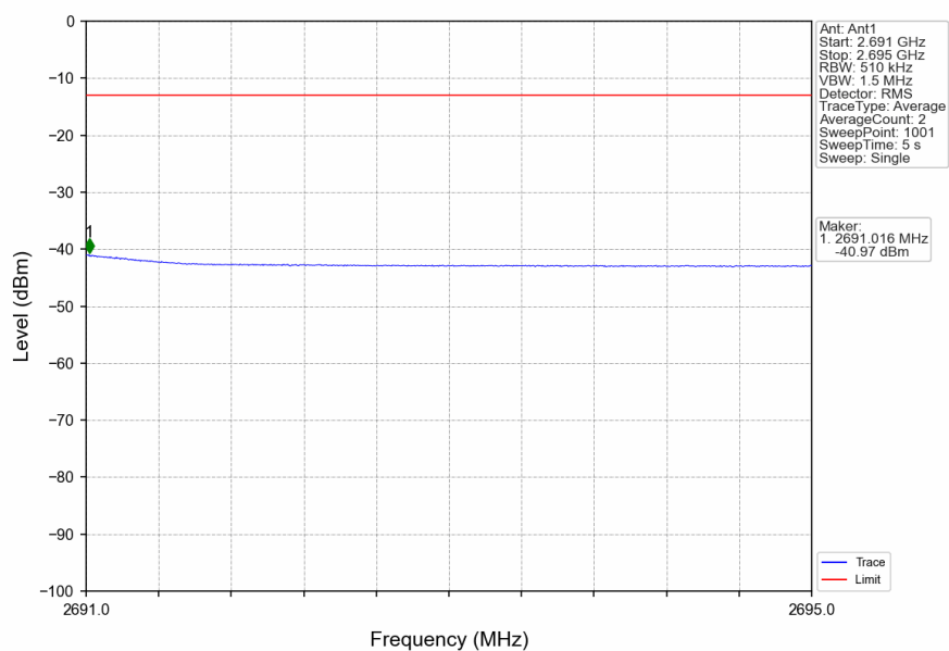
n41_30kHz_SISO_NTNV_90MHz_DFT-s-OFDM_PI/2_BPSK_2644.98MHz_Edge_1RB_Right
