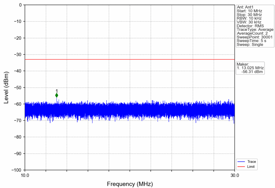
n41_30kHz_SISO_NTNV_80MHz_CP-OFDM_QPSK_2536.02MHz_Edge_1RB_Left
