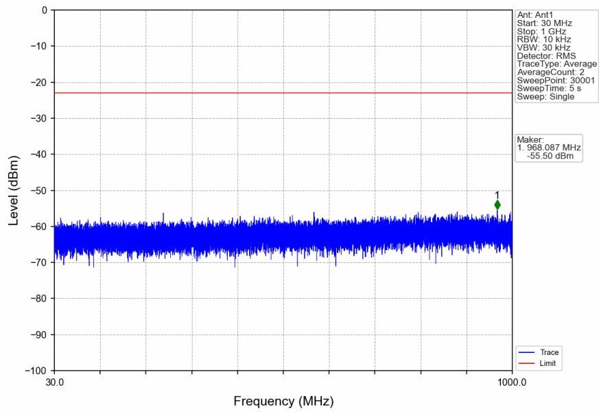
n41_30kHz_SISO_NTNV_80MHz_CP-OFDM_QPSK_2536.02MHz_Edge_1RB_Left
