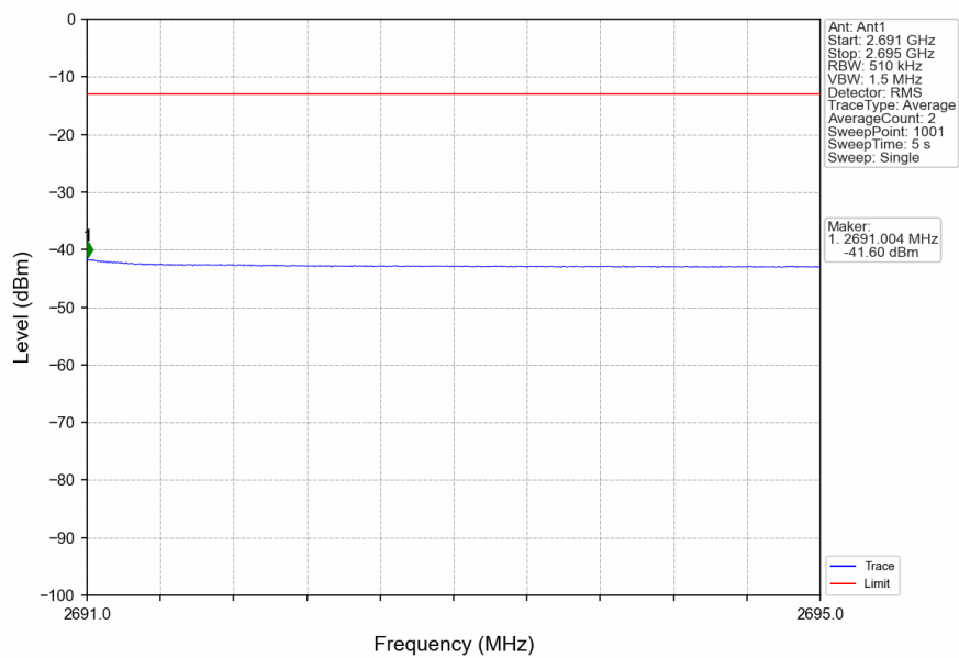
n41_30kHz_SISO_NTNV_80MHz_CP-OFDM_QPSK_2649.99MHz_Inner_1RB_Right
