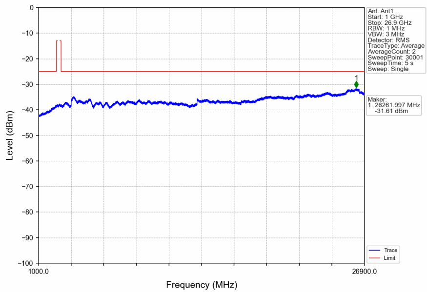
n41_30kHz_SISO_NTNV_90MHz_DFT-s-OFDM_QPSK_2541MHz_Edge_1RB_Left
