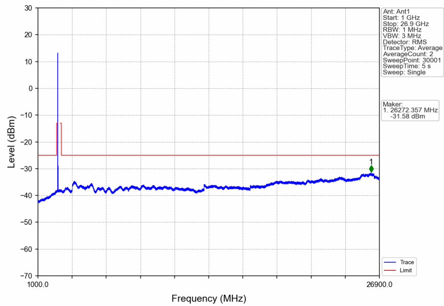
n41_30kHz_SISO_NTNV_80MHz_CP-OFDM_QPSK_2536.02MHz_Edge_1RB_Left
