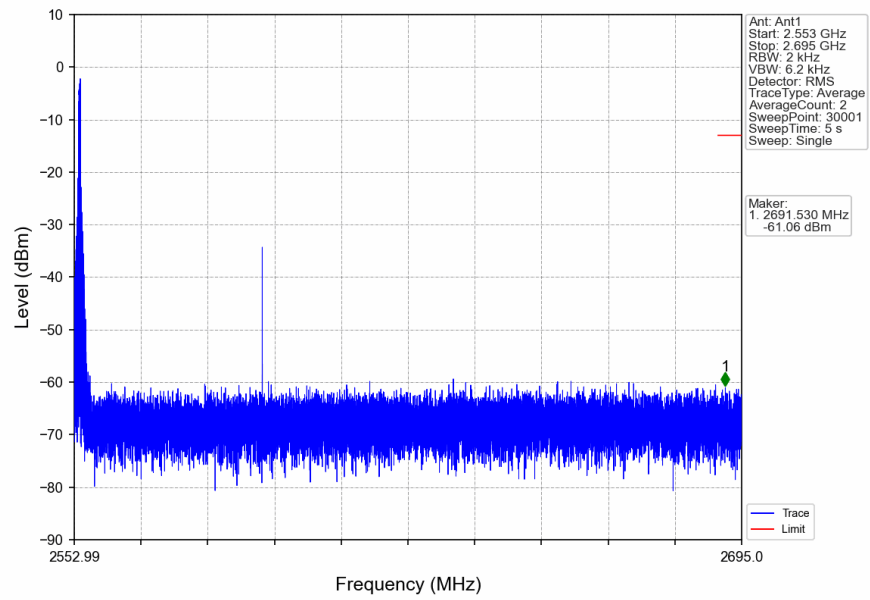
n41_30kHz_SISO_NTNV_80MHz_CP-OFDM_QPSK_2592.99MHz_Edge_1RB_Left
