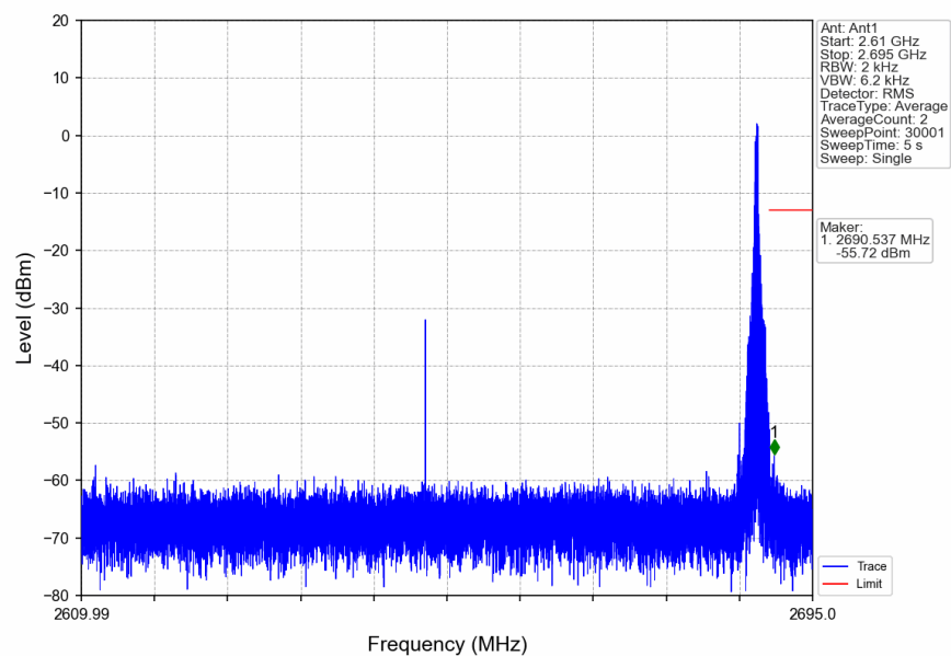
n41_30kHz_SISO_NTNV_80MHz_CP-OFDM_QPSK_2649.99MHz_Inner_1RB_Right
