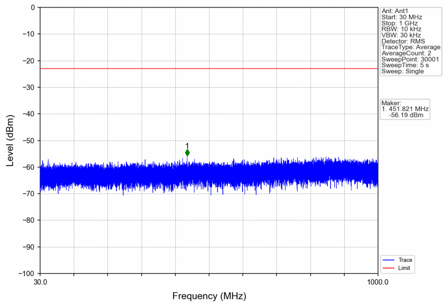
n41_30kHz_SISO_NTNV_80MHz_CP-OFDM_QPSK_2592.99MHz_Edge_1RB_Left
