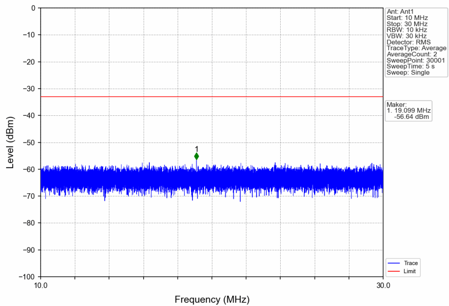
n41_30kHz_SISO_NTNV_90MHz_DFT-s-OFDM_QPSK_2541MHz_Edge_1RB_Left
