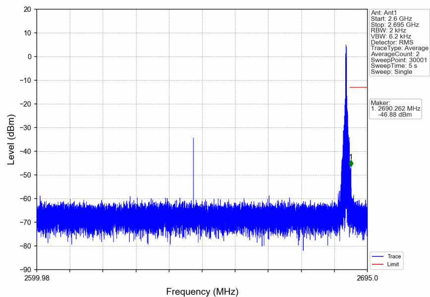
n41_30kHz_SISO_NTNV_90MHz_DFT-s-OFDM_PI/2_BPSK_2644.98MHz_Edge_1RB_Right
